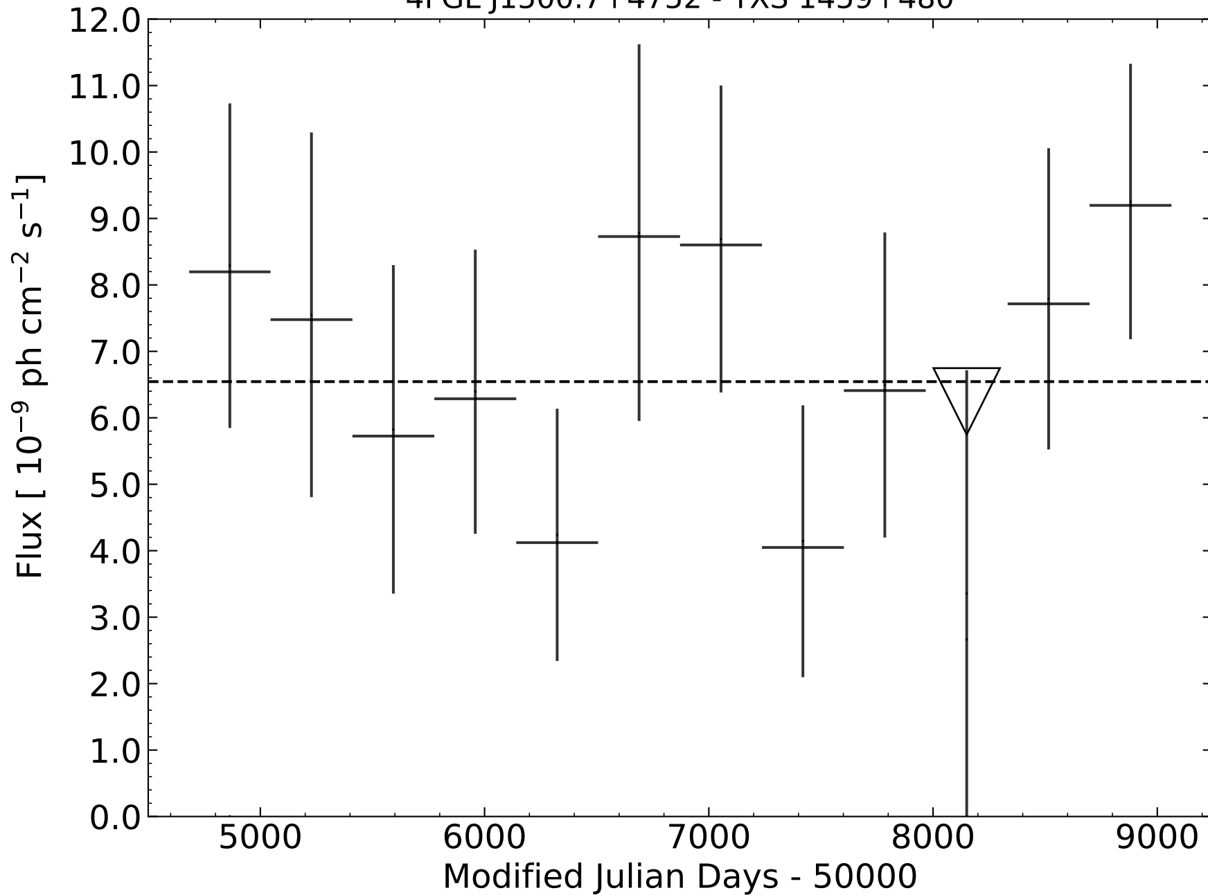
4FGL J1500.7+4752 - TXS 1459+480
