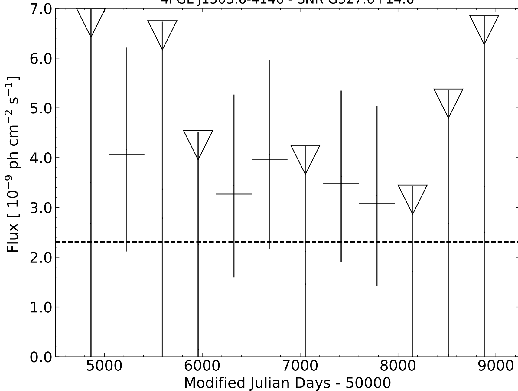
4FGL J1503.6-4146 - SNR G327.6+14.6
