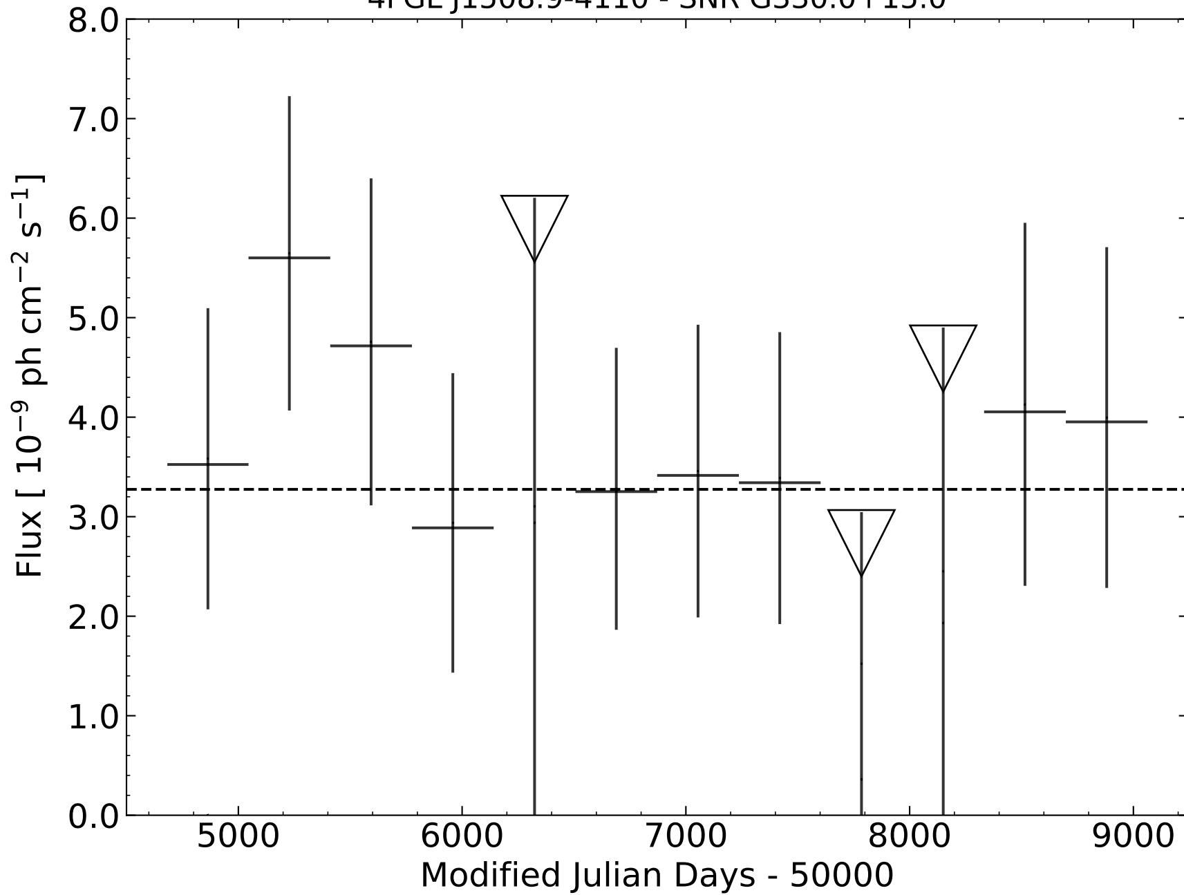
4FGL J1508.9-4110 - SNR G330.0+15.0
