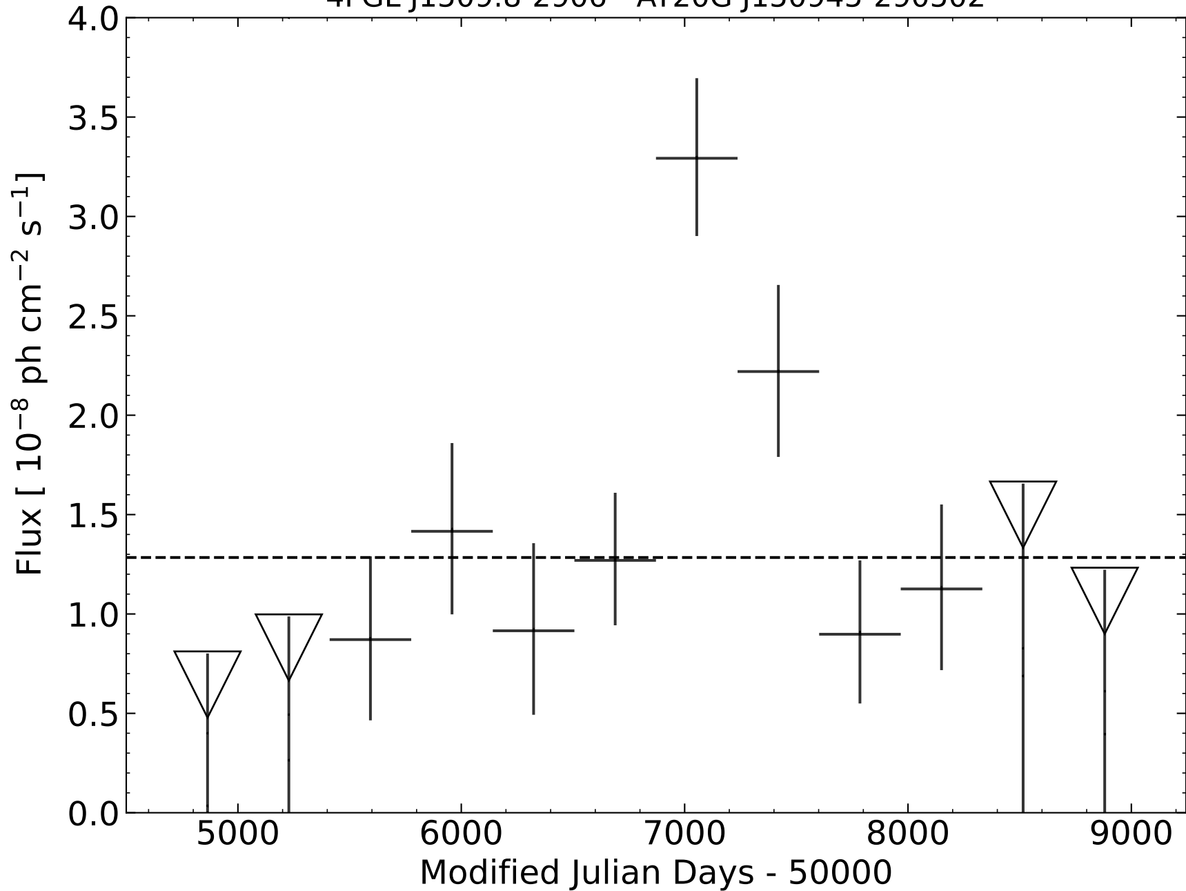
4FGL J1509.8-2906 - AT20G J150945-290502
