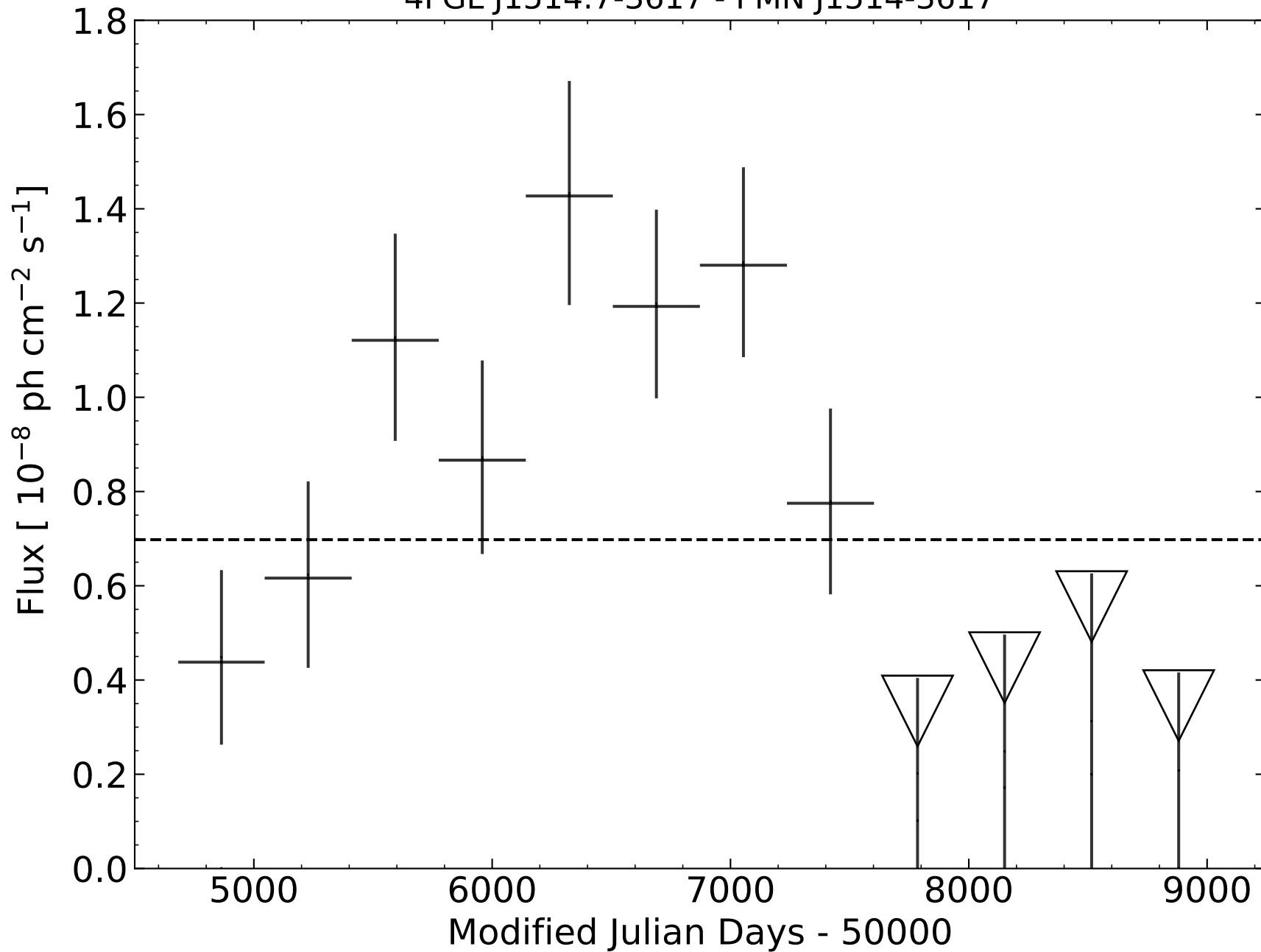
4FGL J1514.7-3617 - PMN J1514-3617
