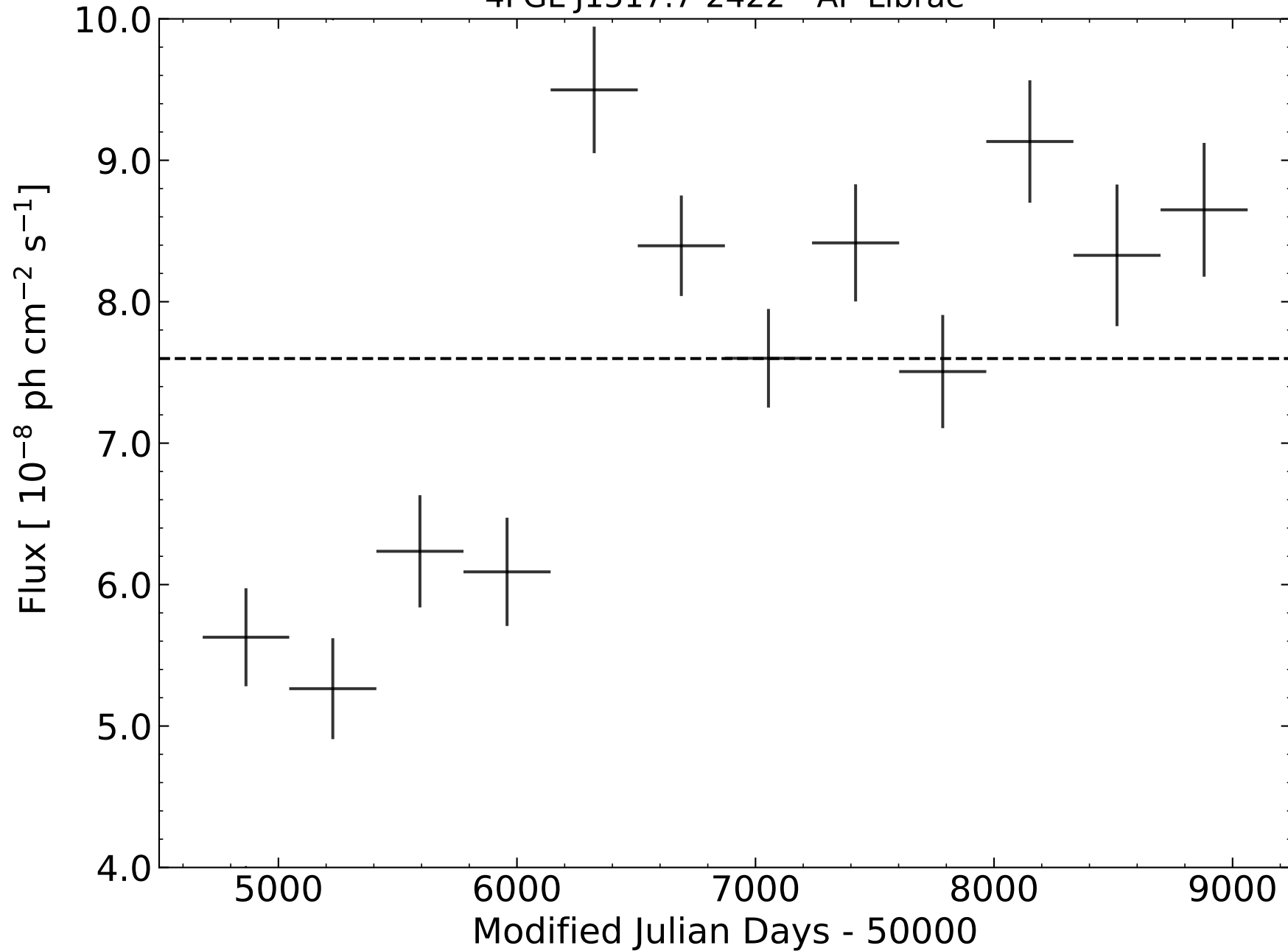
4FGL J1517.7-2422 - AP Librae
