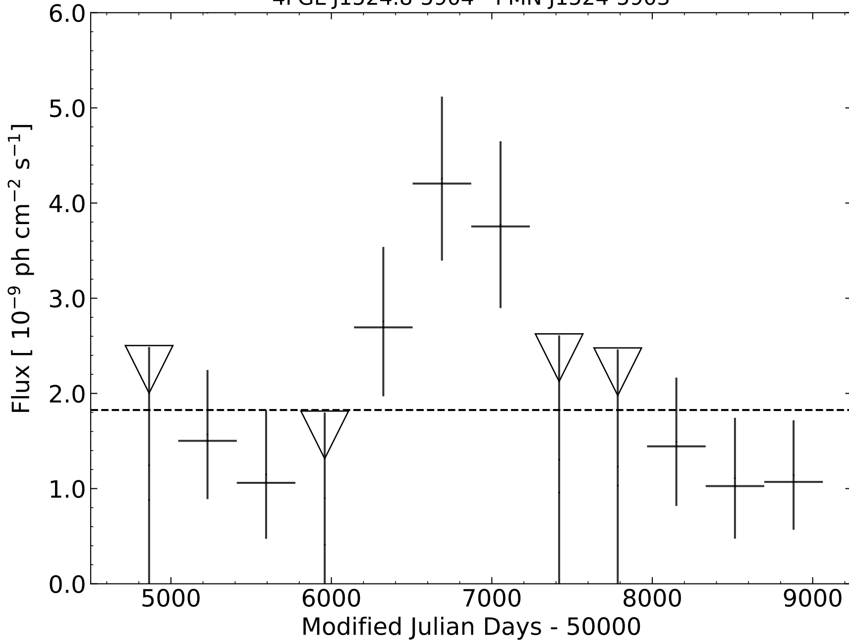
4FGL J1524.8-5904 - PMN J1524-5903
