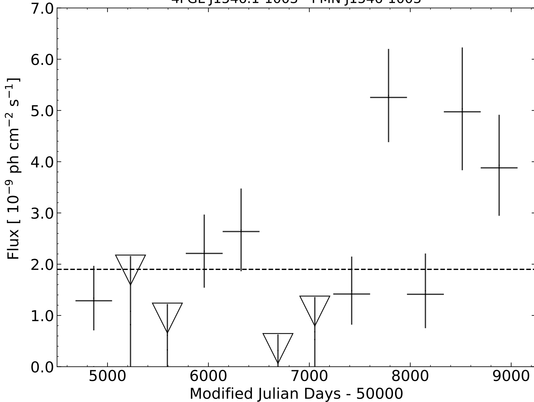
4FGL J1546.1-1003 - PMN J1546-1003
