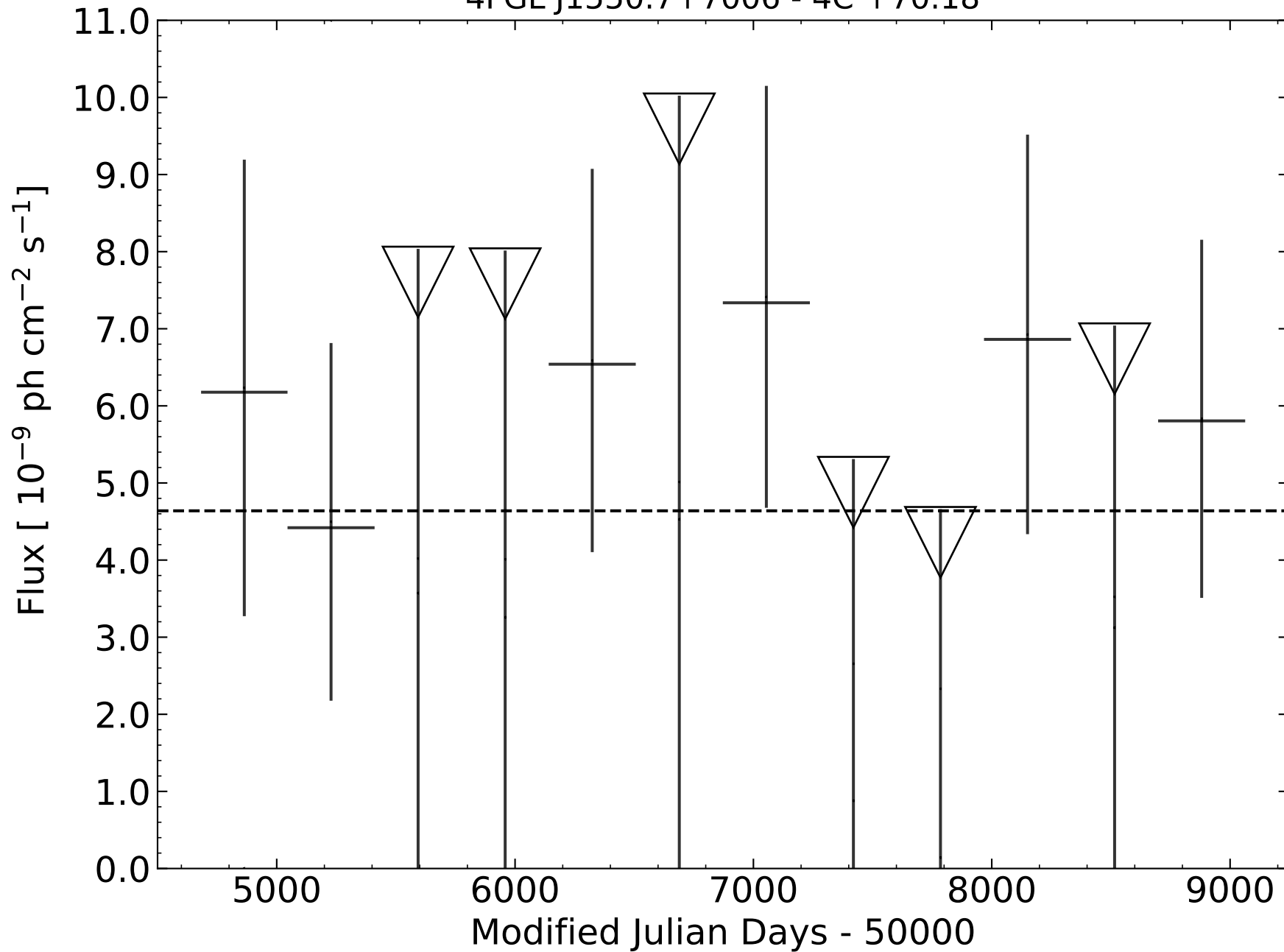
4FGL J1550.7+7006 - 4C +70.18
