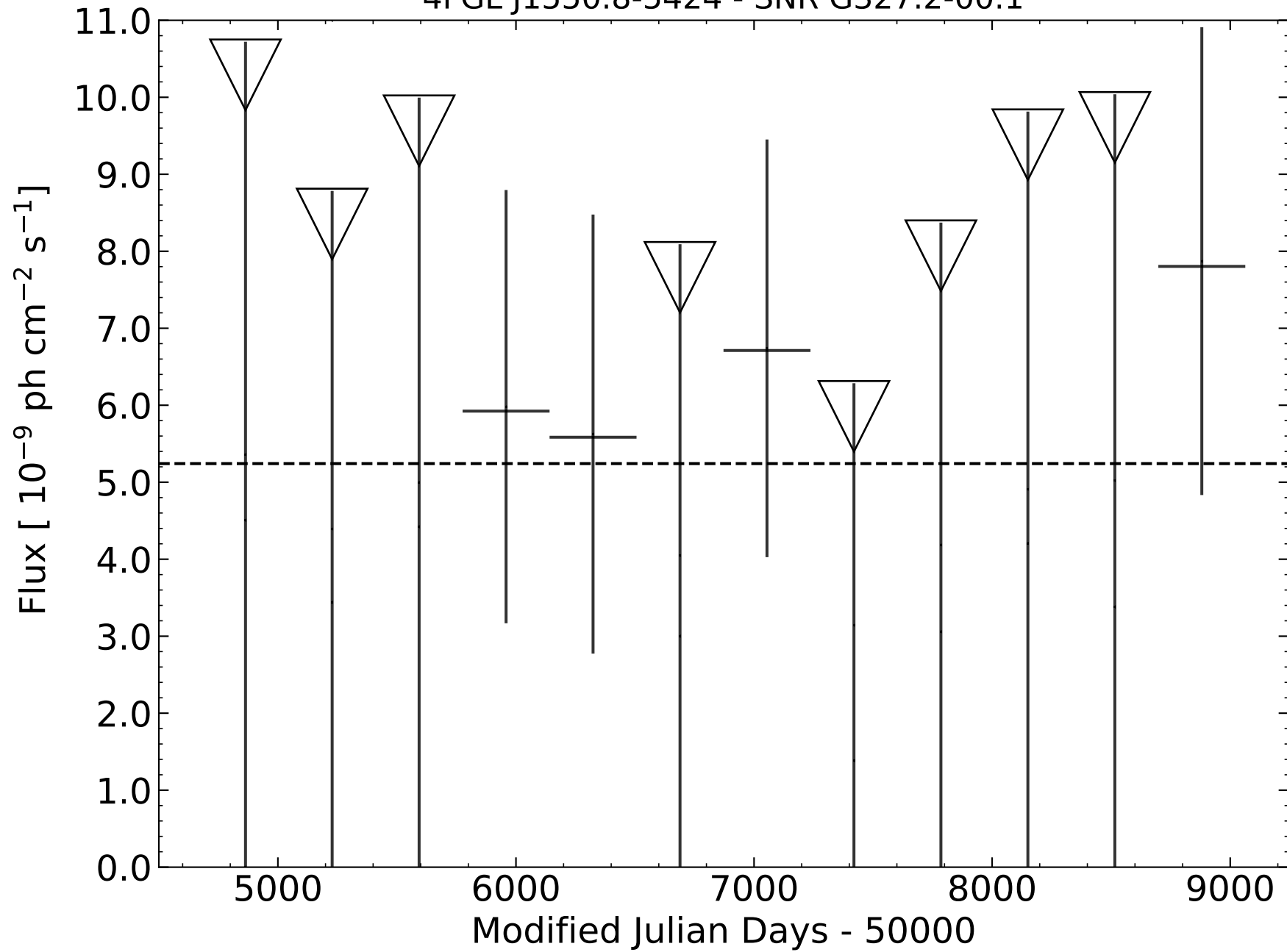
4FGL J1550.8-5424 - SNR G327.2-00.1
