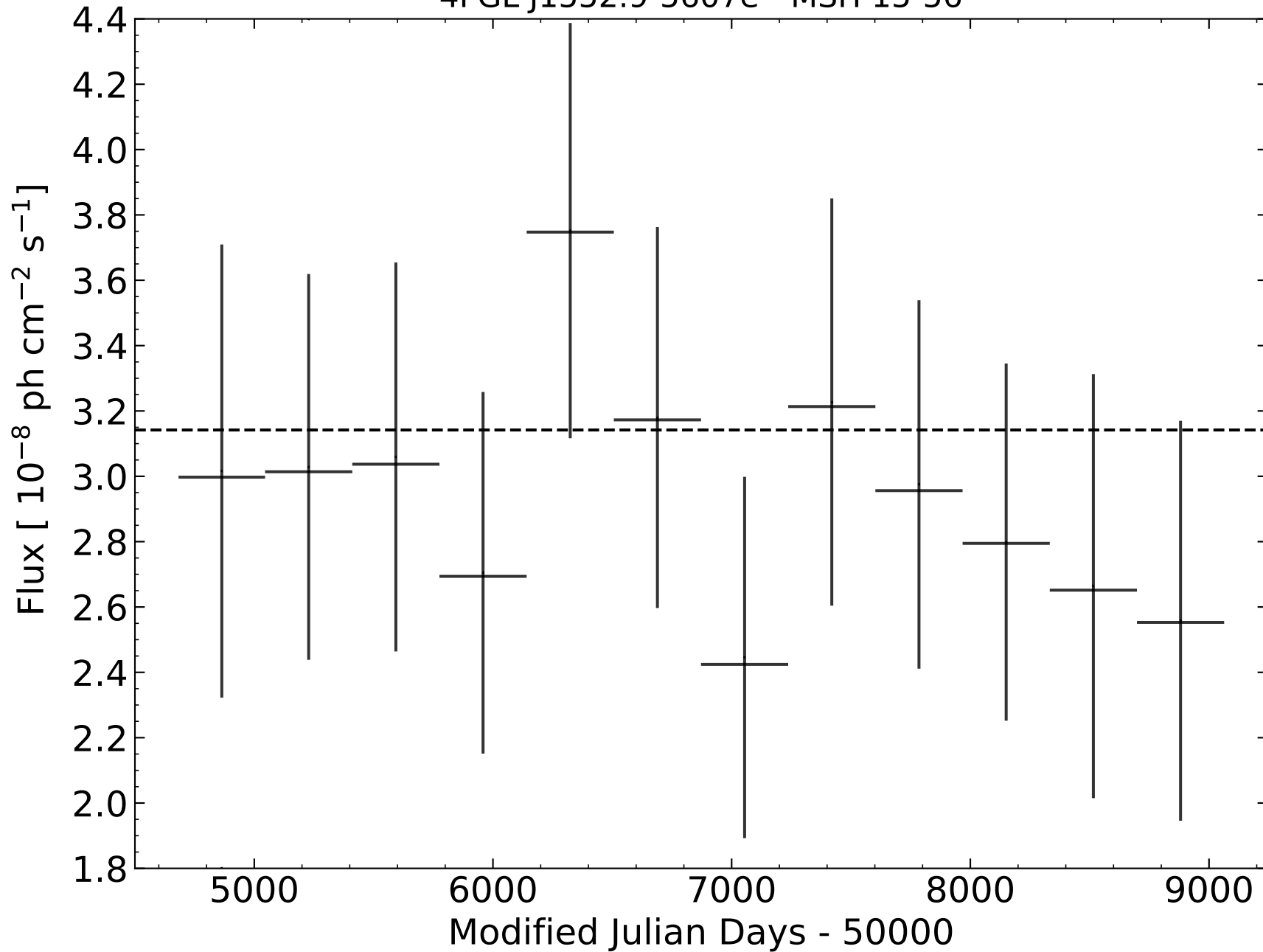
4FGL J1552.9-5607e - MSH 15-56
