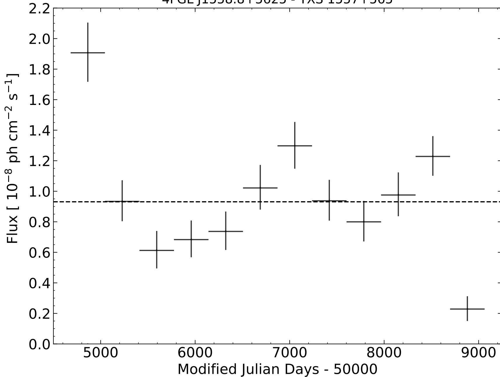
4FGL J1558.8+5625 - TXS 1557+565
