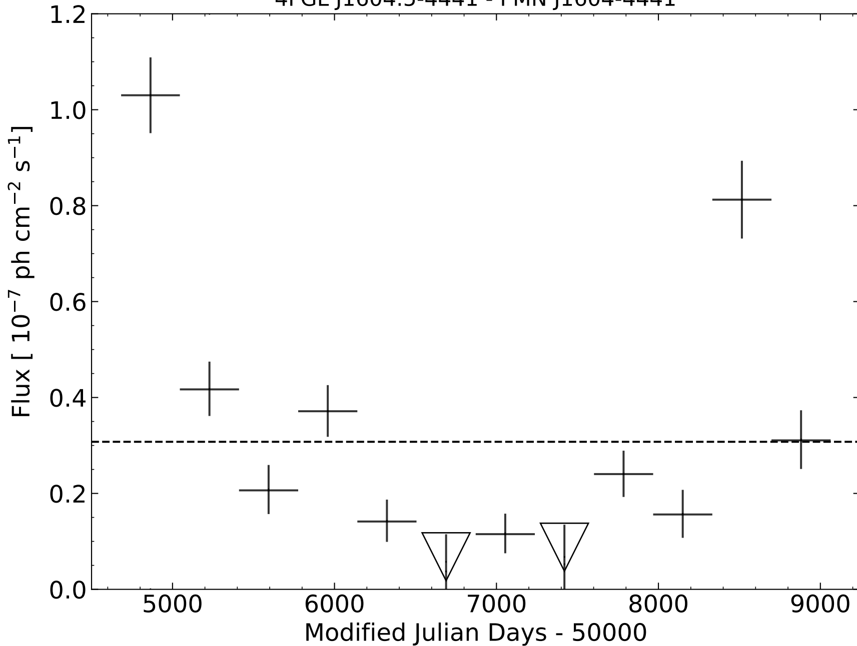
4FGL J1604.5-4441 - PMN J1604-4441
