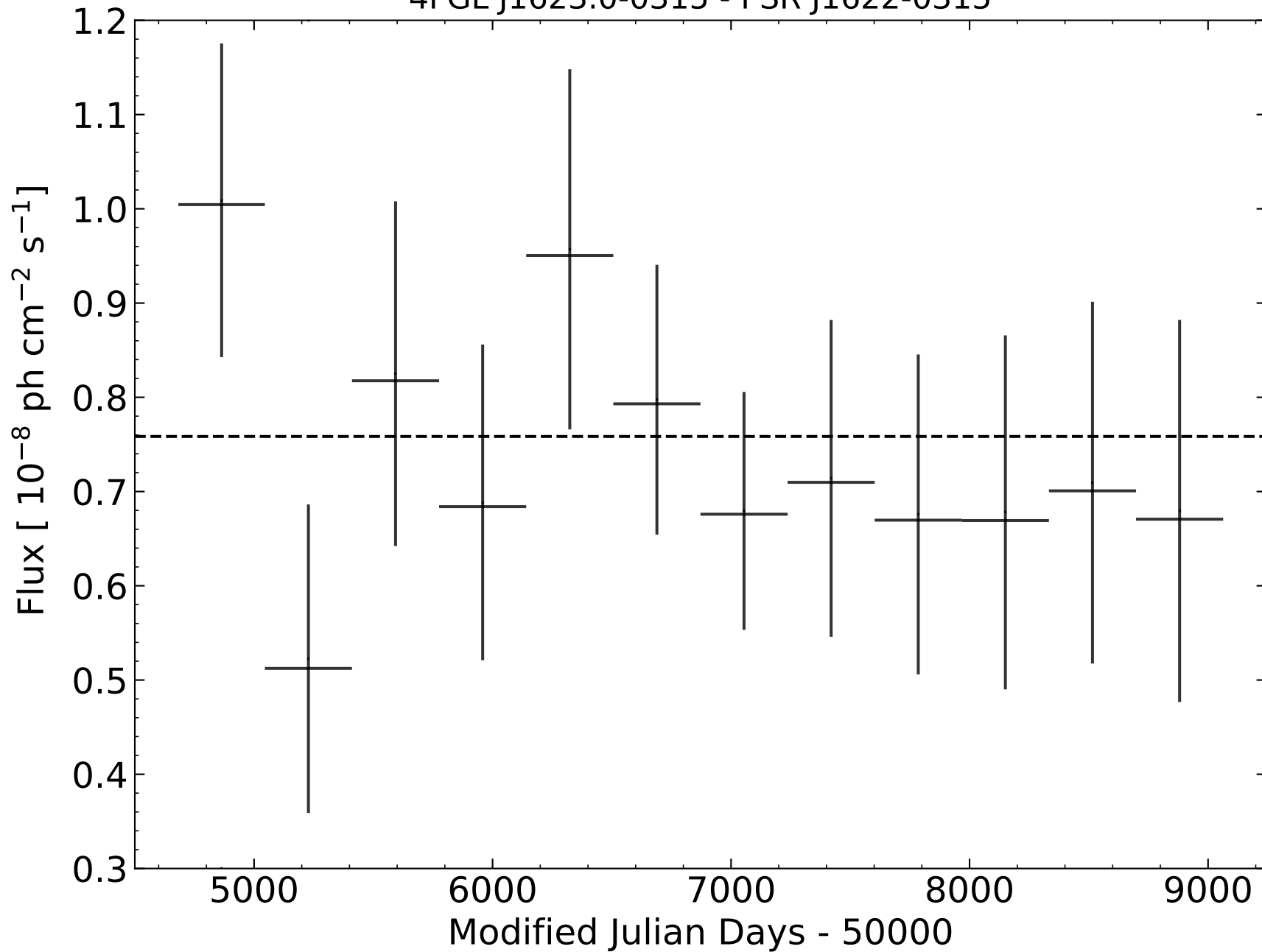
4FGL J1623.0-0315 - PSR J1622-0315
