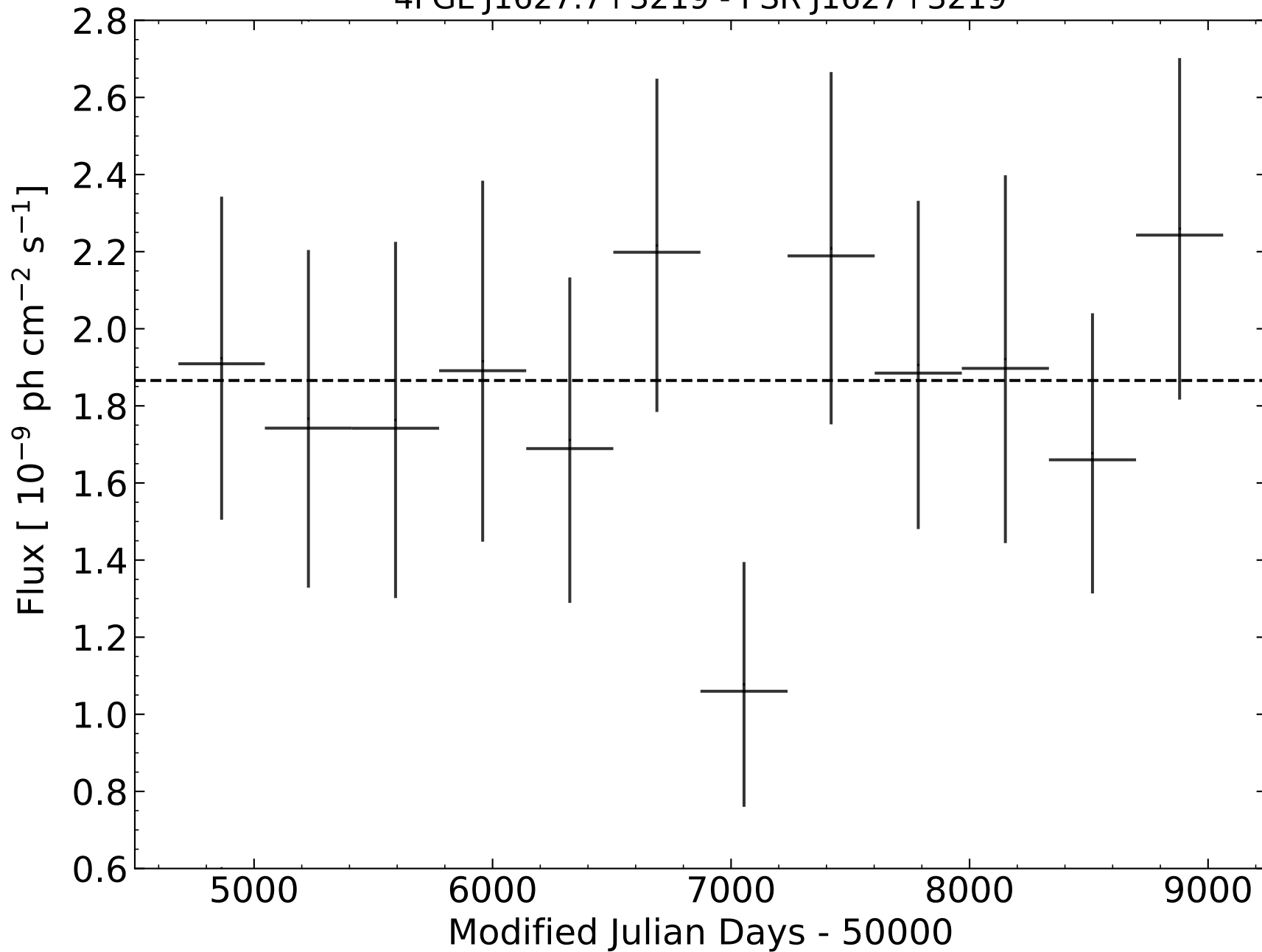
4FGL J1627.7+3219 - PSR J1627+3219
