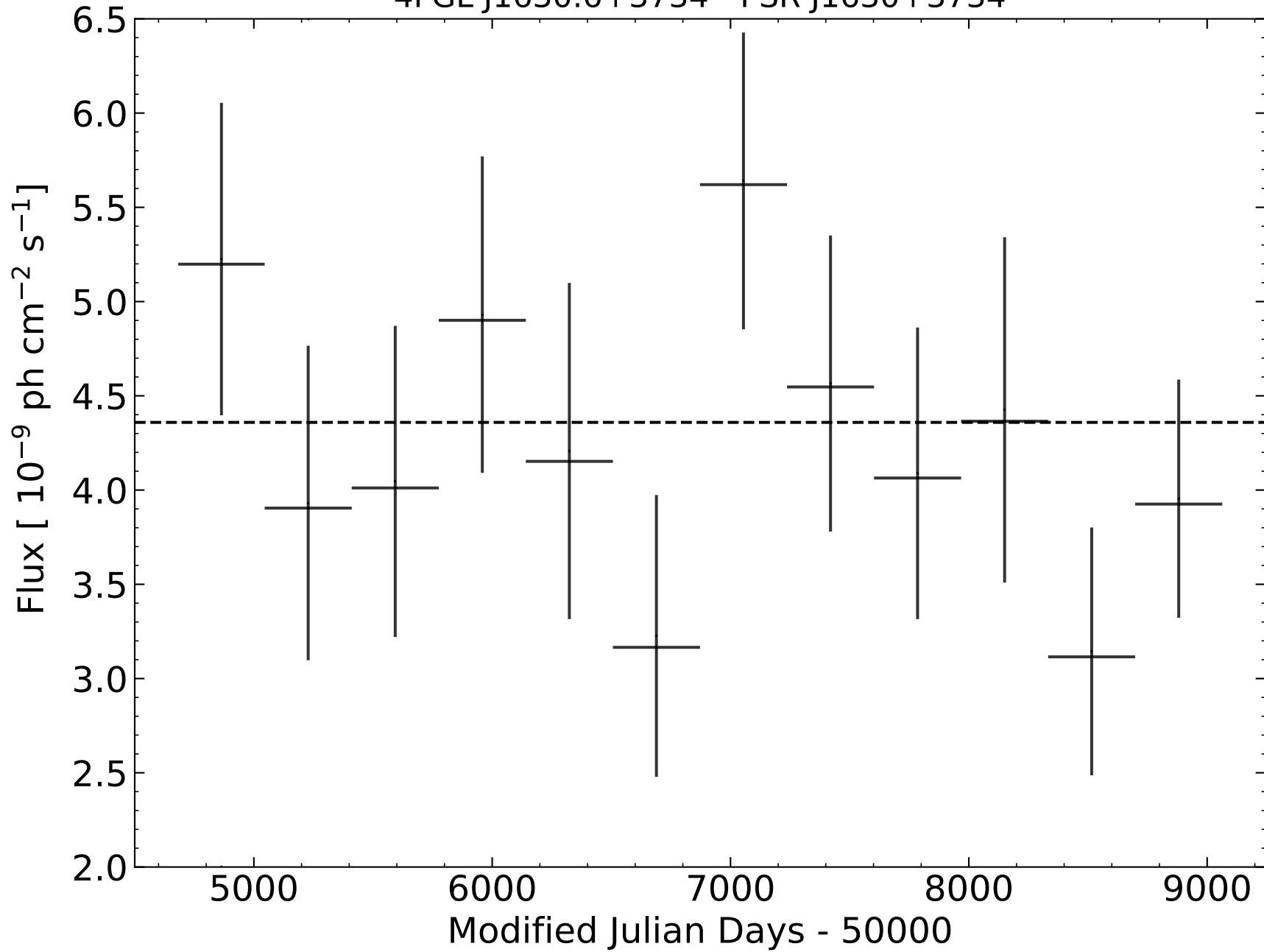
4FGL J1630.6+3734 - PSR J1630+3734
