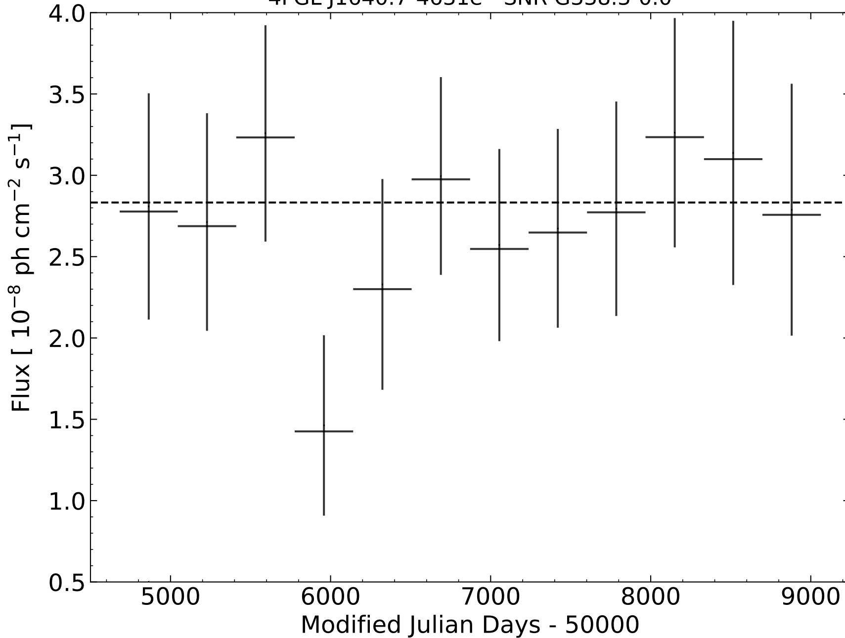
4FGL J1640.7-4631e - SNR G338.3-0.0
