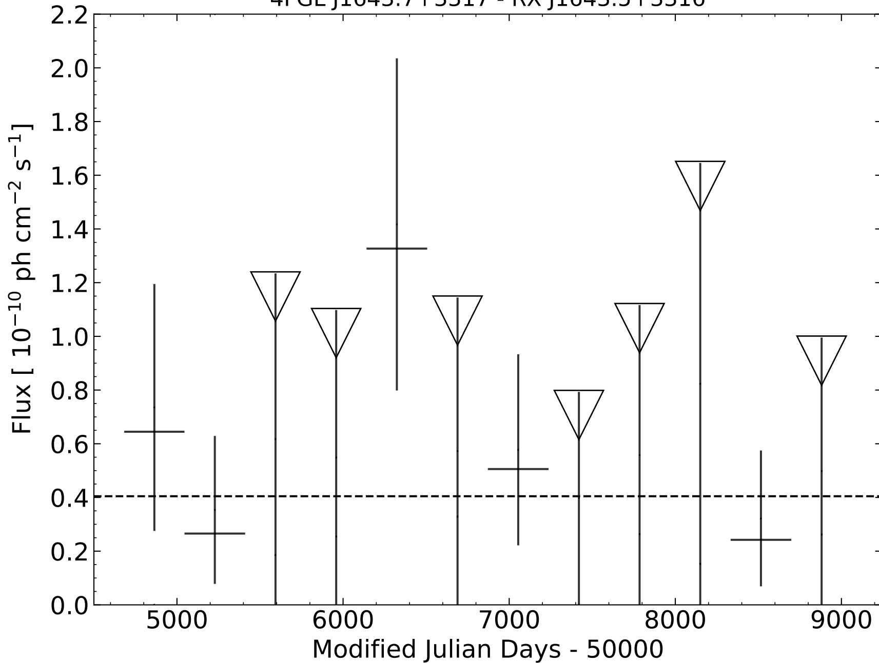
4FGL J1643.7+3317 - RX J1643.5+3316
