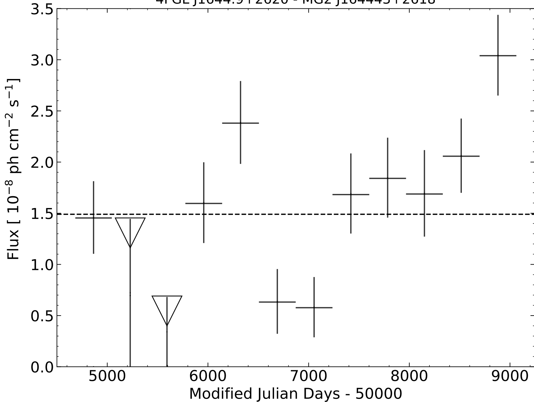
4FGL J1644.9+2620 - MG2 J164443+2618
