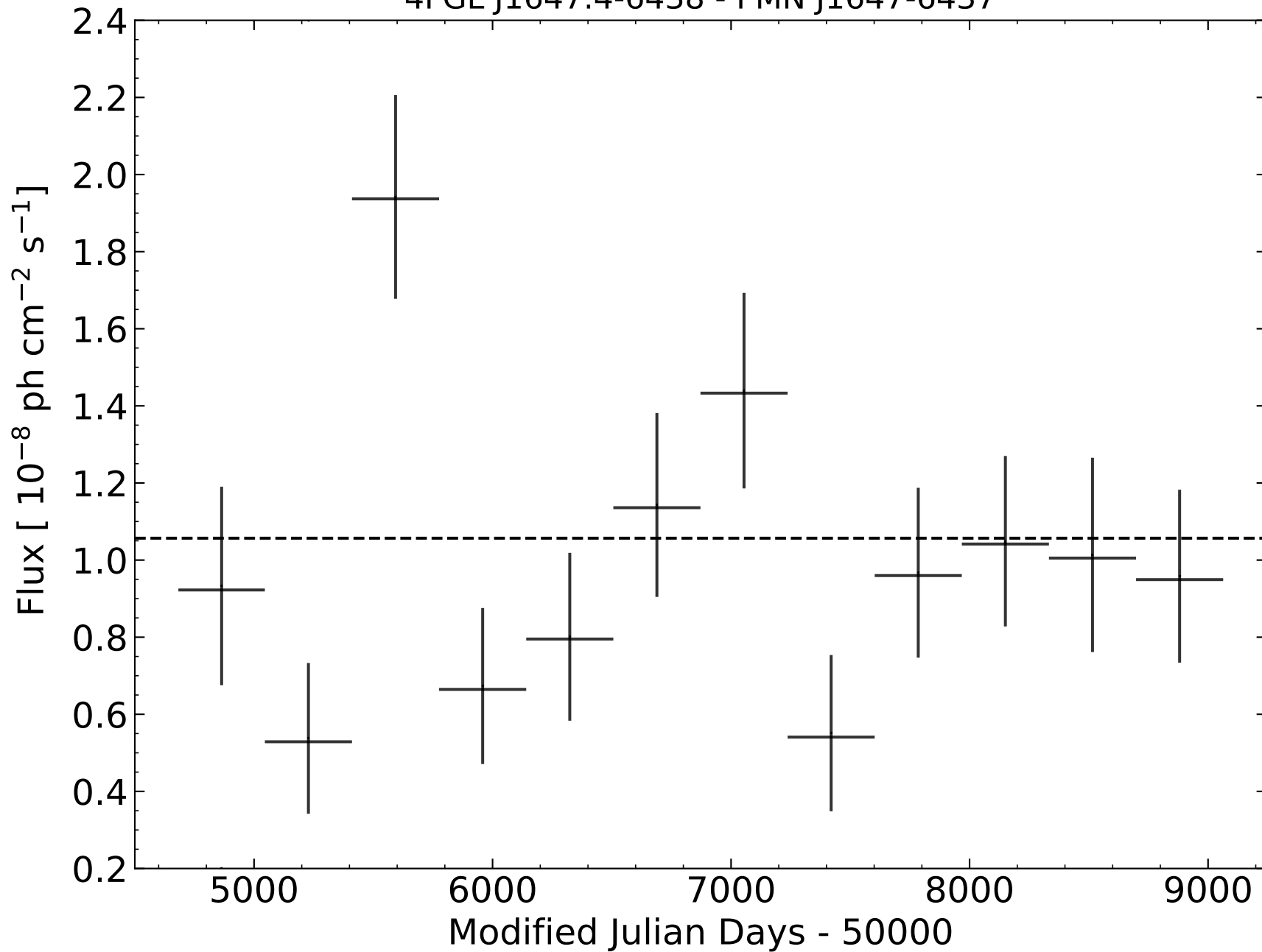
4FGL J1647.4-6438 - PMN J1647-6437
