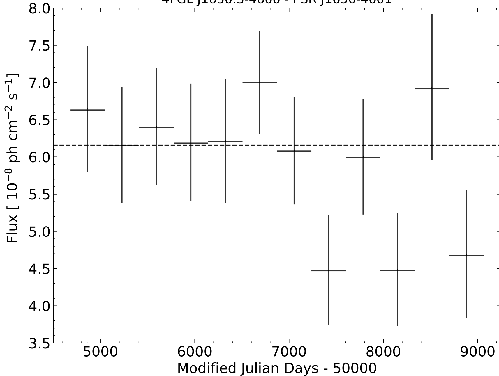
4FGL J1650.3-4600 - PSR J1650-4601
