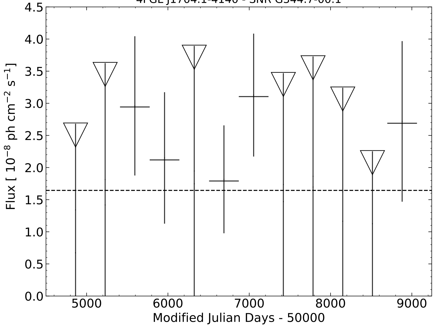
4FGL J1704.1-4140 - SNR G344.7-00.1
