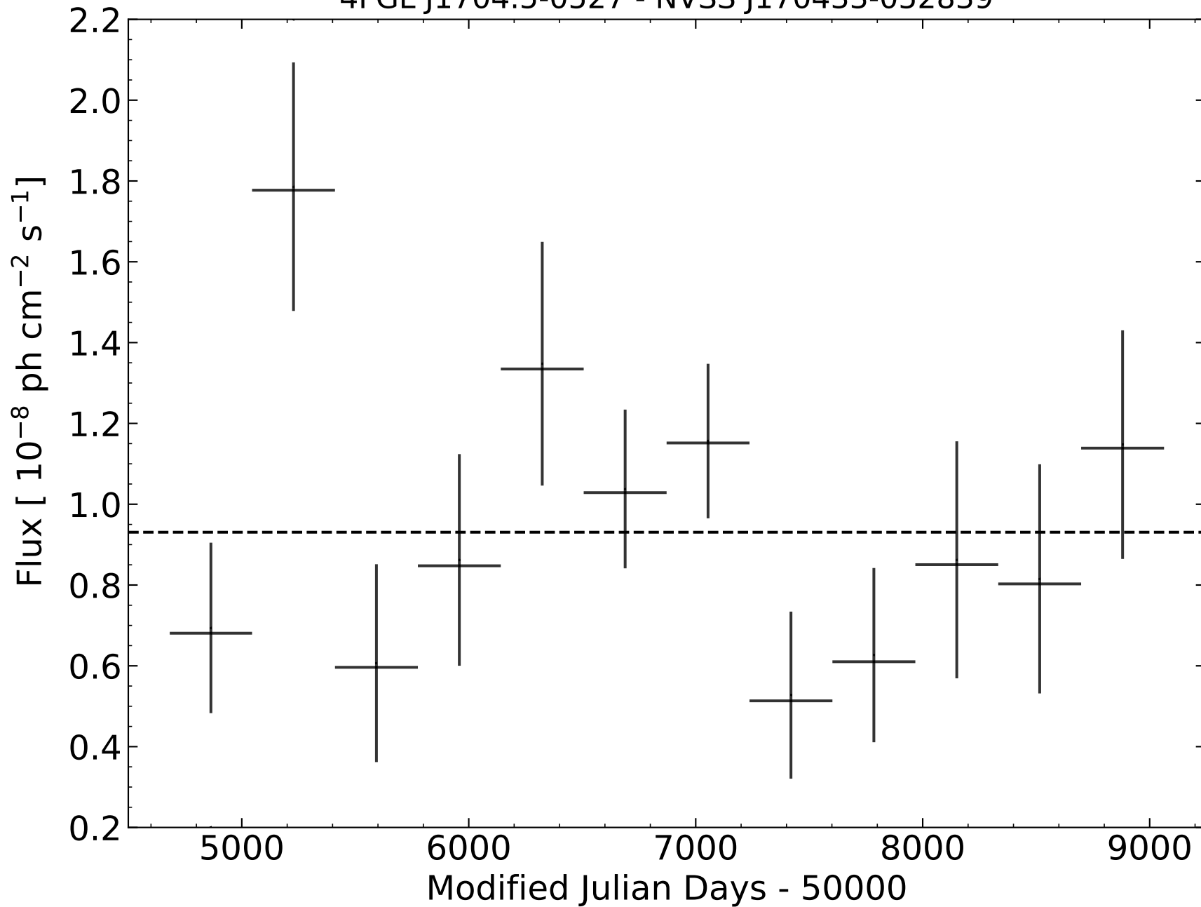
4FGL J1704.5-0527 - NVSS J170433-052839
