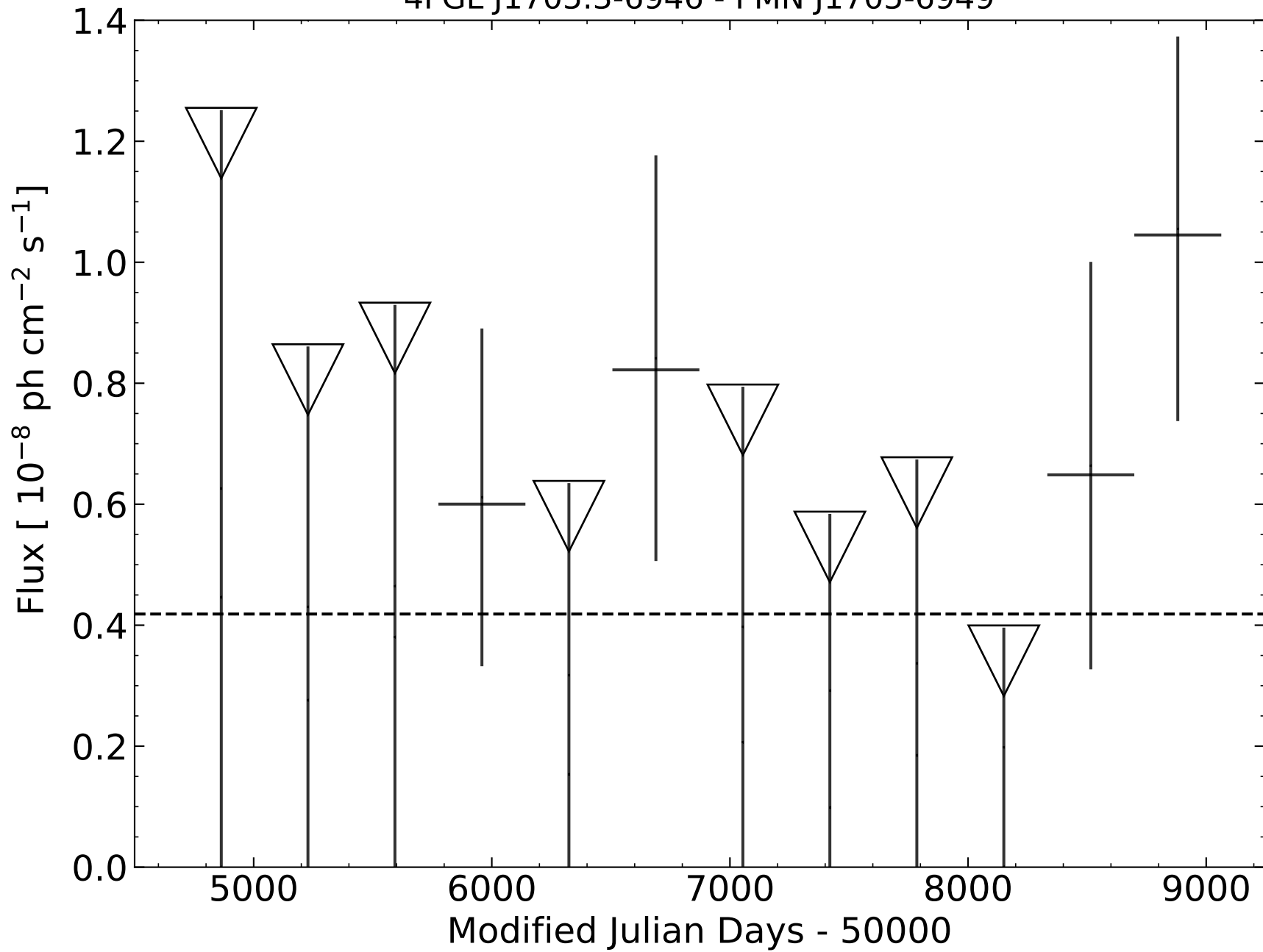
4FGL J1705.3-6946 - PMN J1705-6949
