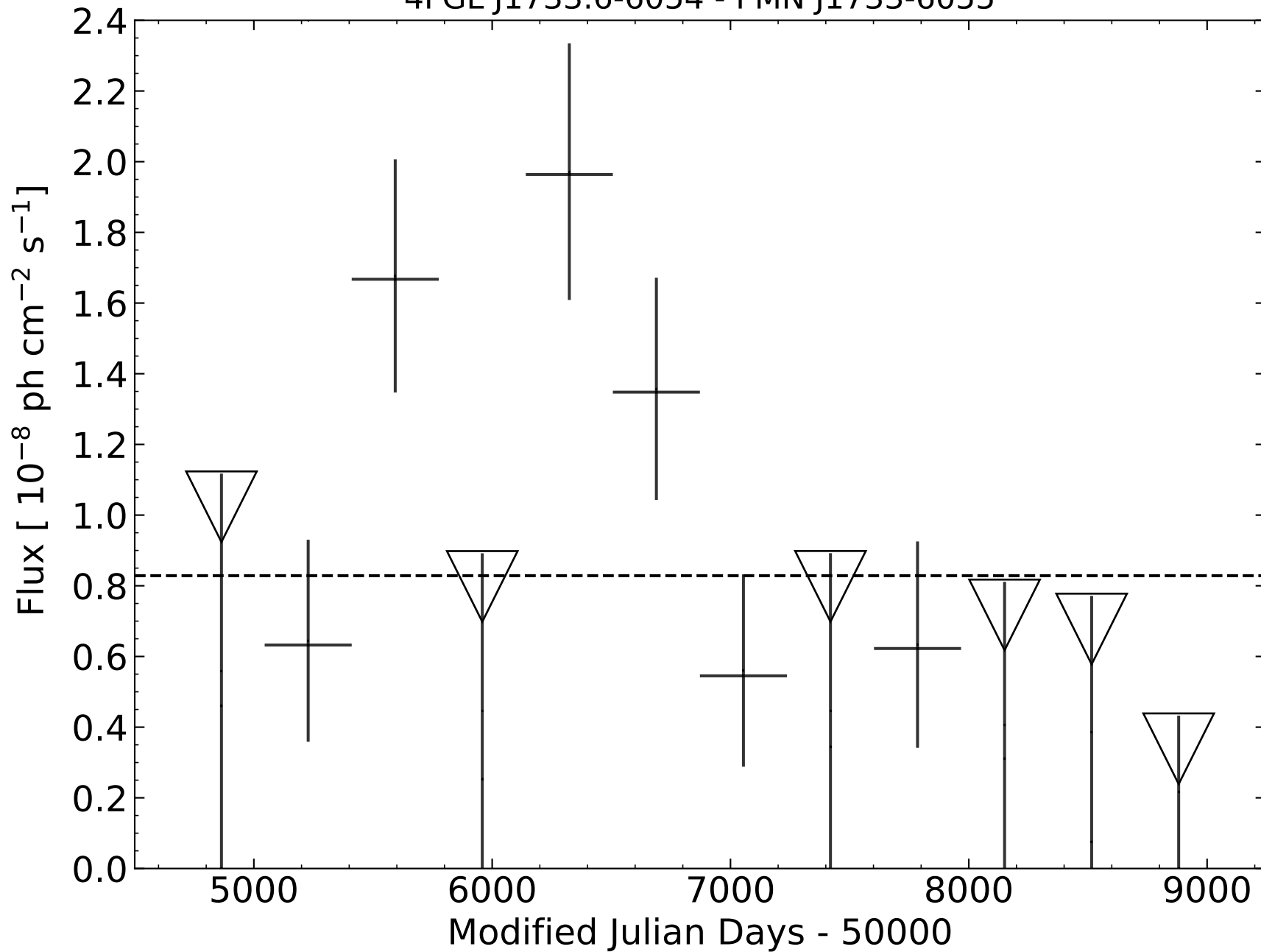
4FGL J1733.6-6054 - PMN J1733-6055
