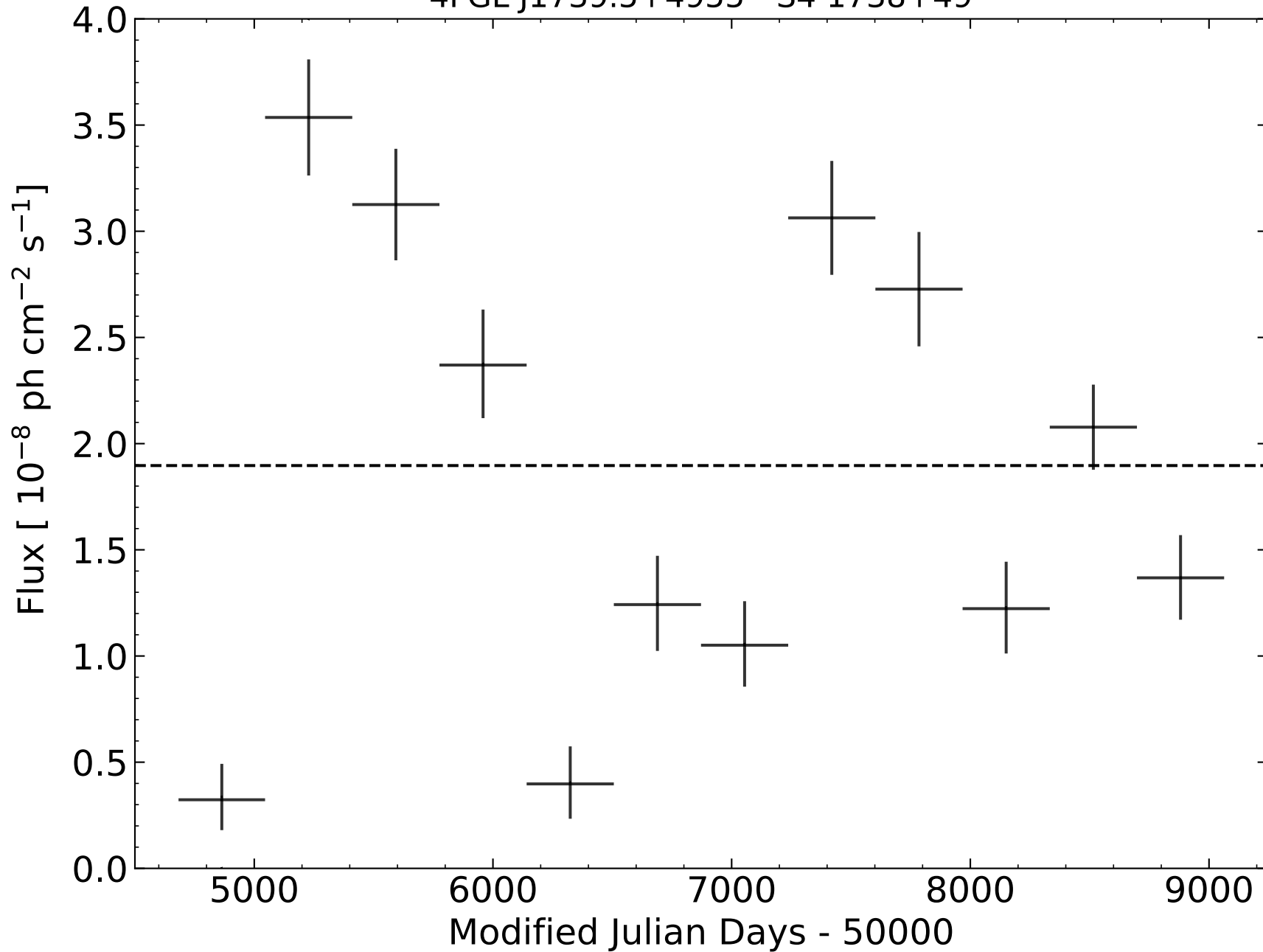
4FGL J1739.5+4955 - S4 1738+49
