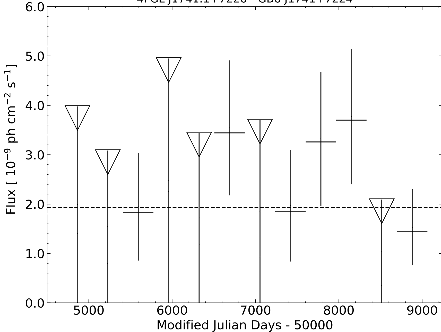
4FGL J1741.1+7226 - GB6 J1741+7224
