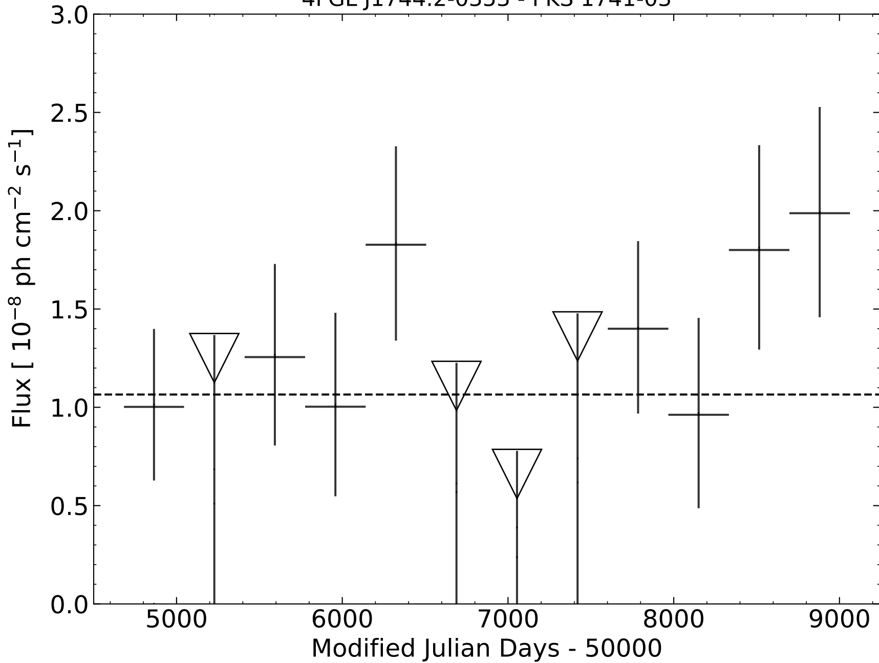
4FGL J1744.2-0353 - PKS 1741-03
