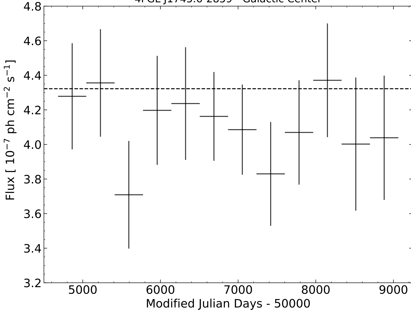
4FGL J1745.6-2859 - Galactic Center
