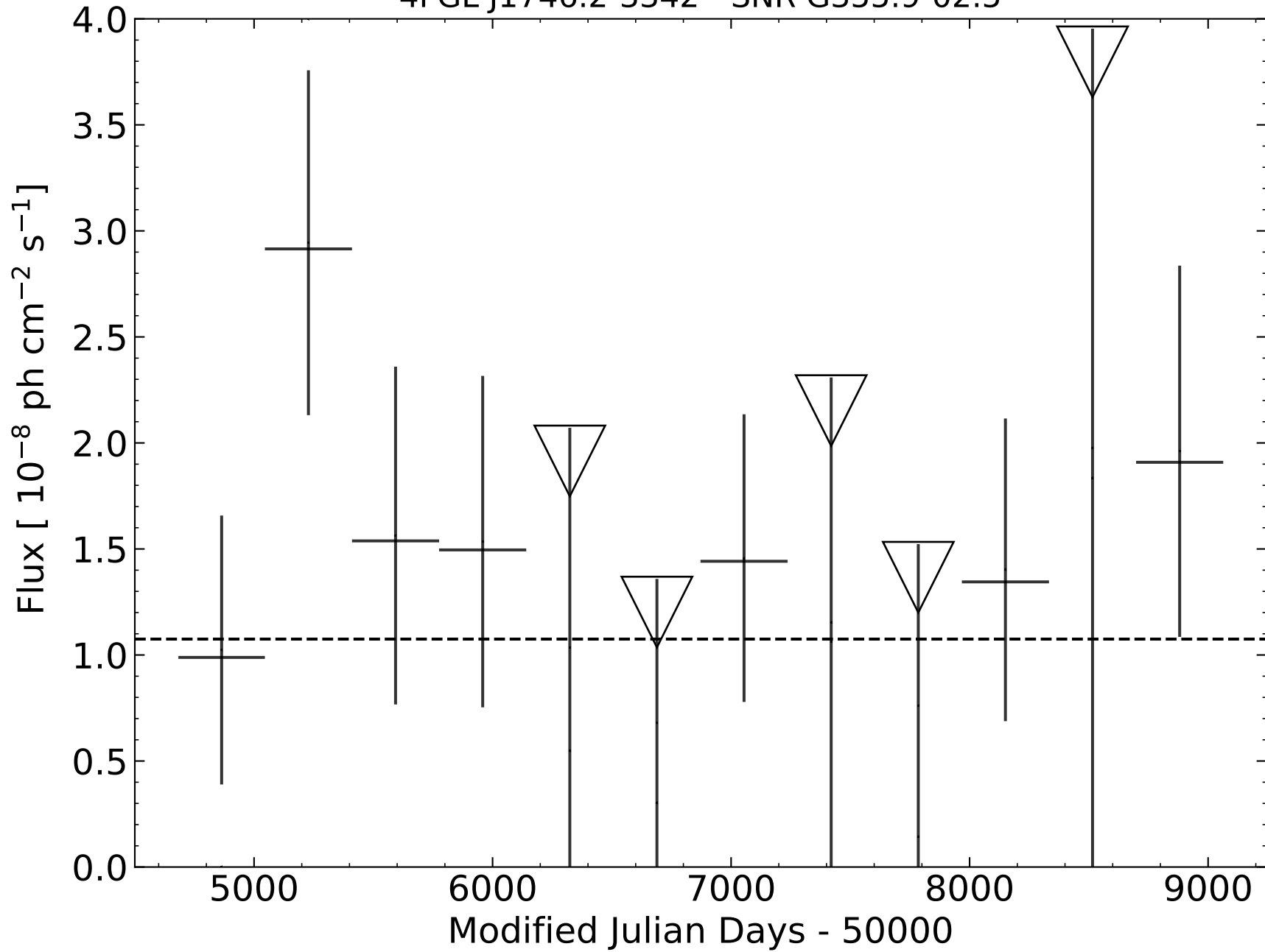
4FGL J1746.2-3342 - SNR G355.9-02.5
