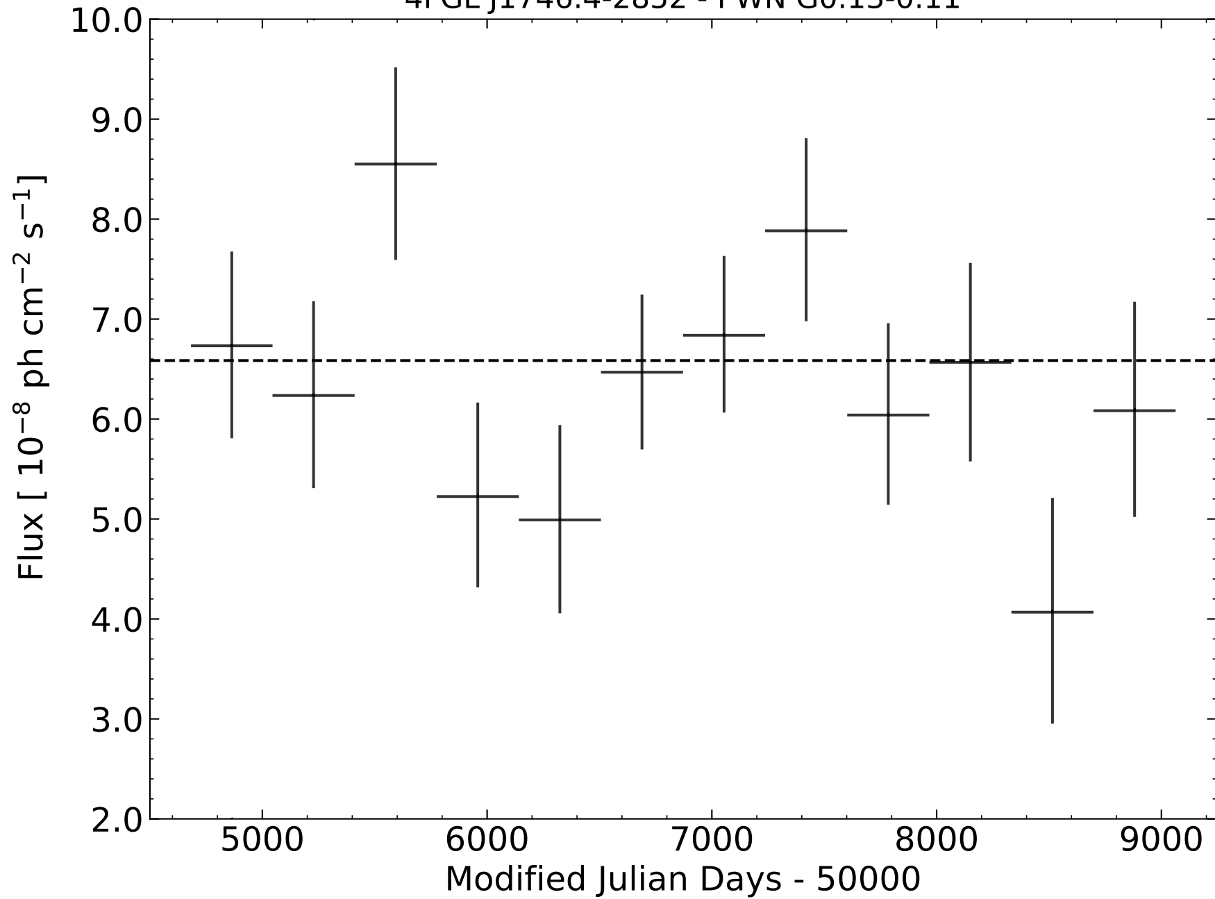
4FGL J1746.4-2852 - PWN G0.13-0.11
