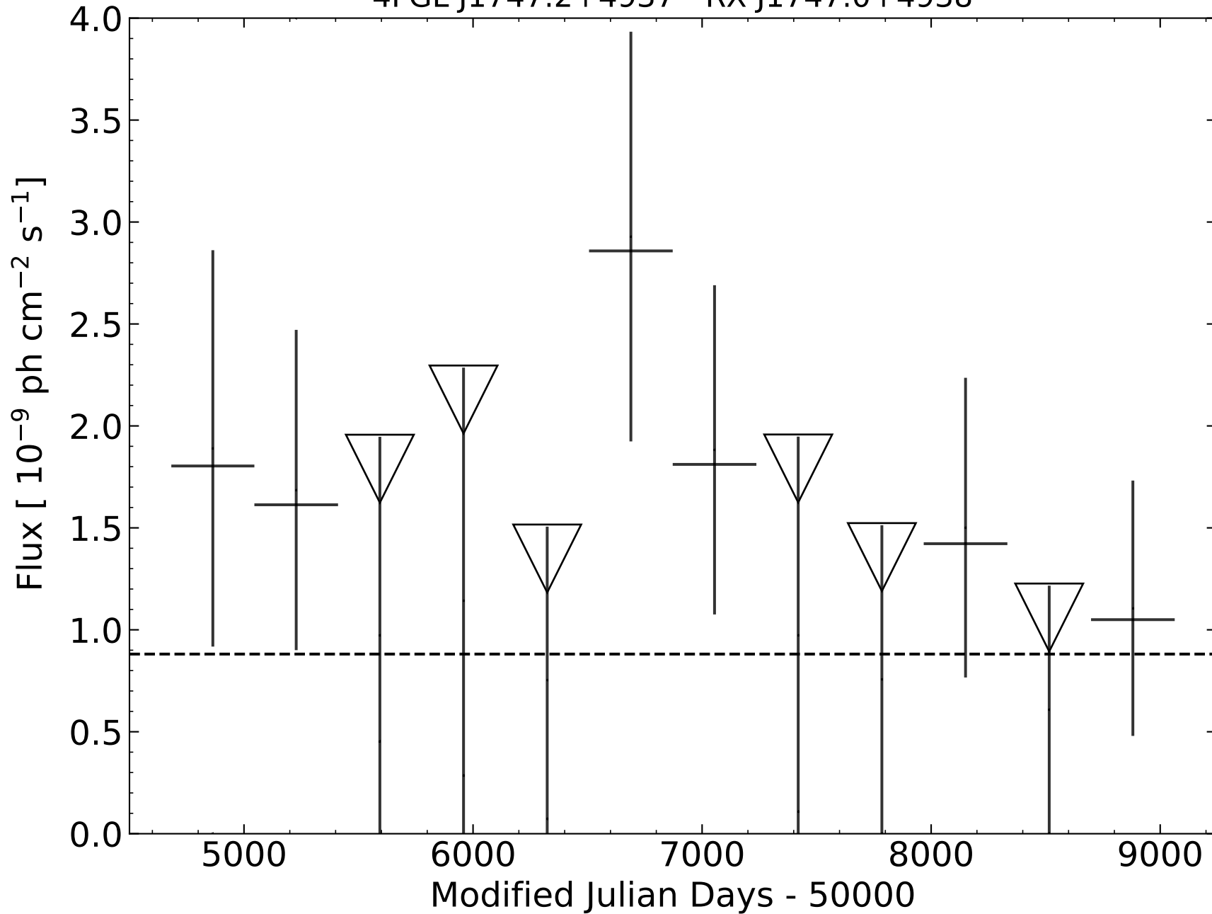
4FGL J1747.2+4937 - RX J1747.0+4938
