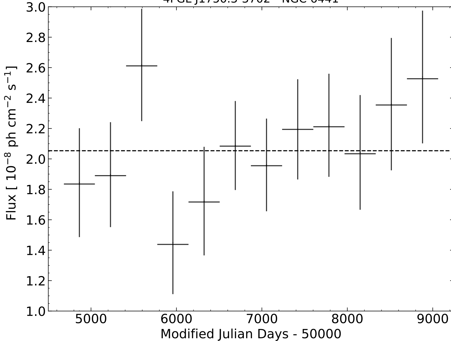
4FGL J1750.3-3702 - NGC 6441
