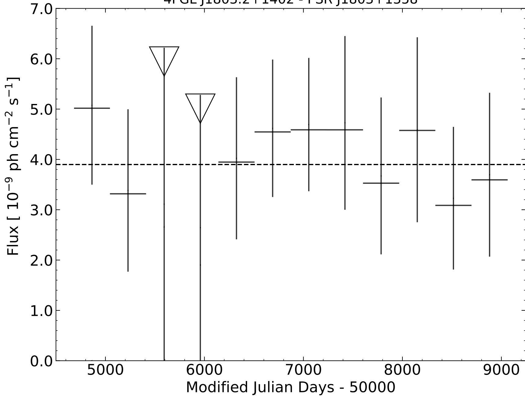
4FGL J1803.2+1402 - PSR J1803+1358
