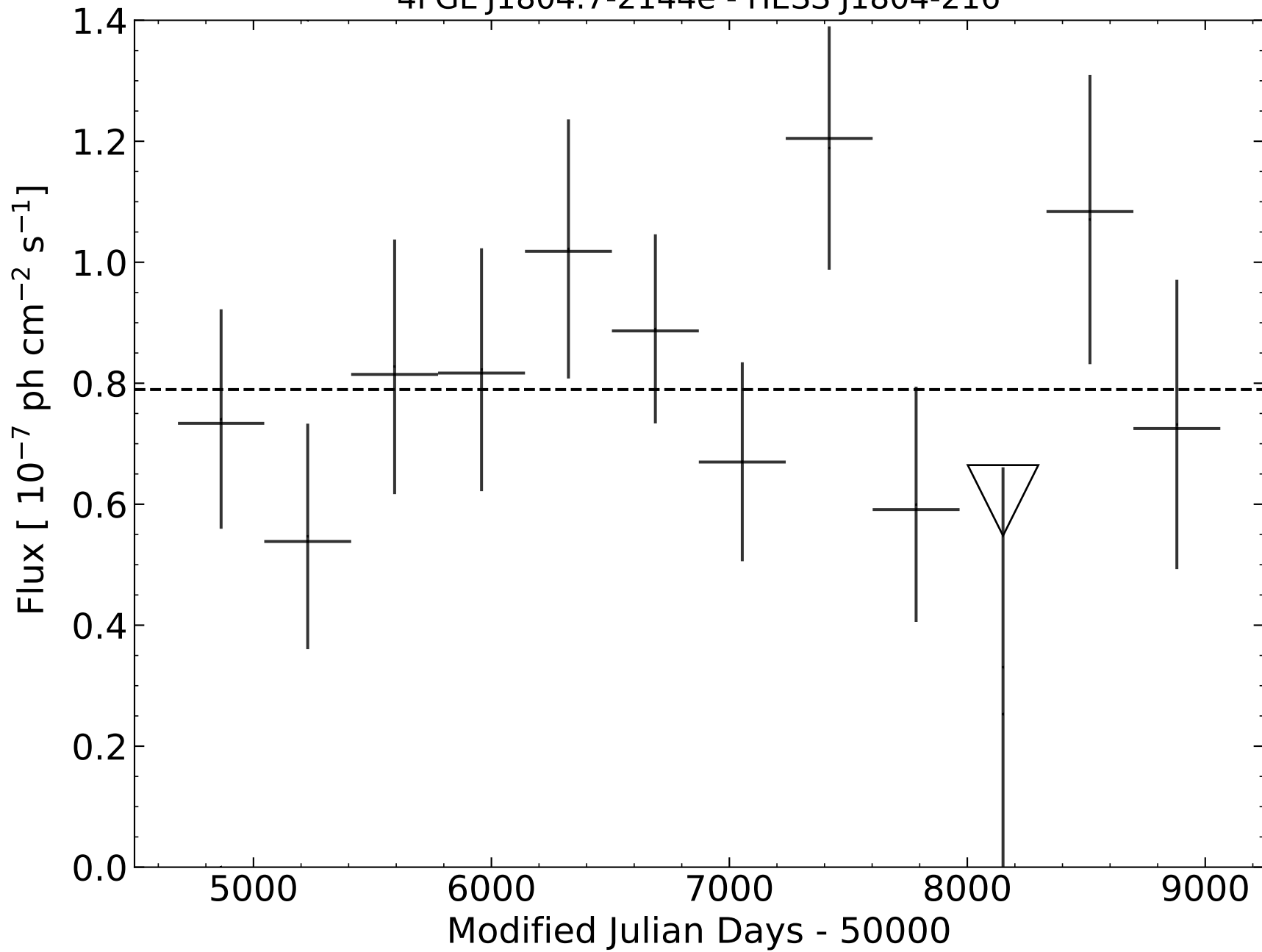
4FGL J1804.7-2144e - HESS J1804-216
