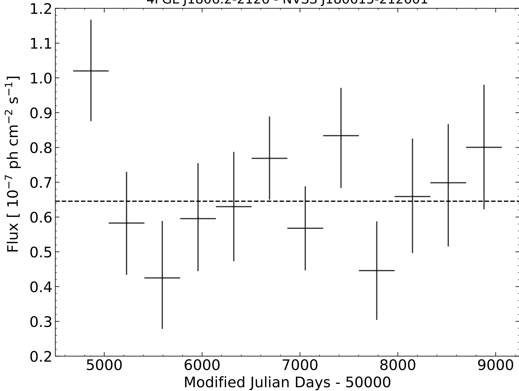
4FGL J1806.2-2126 - NVSS J180615-212601
