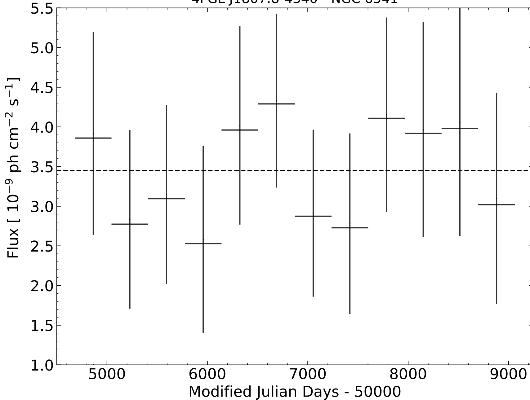
4FGL J1807.8-4340 - NGC 6541
