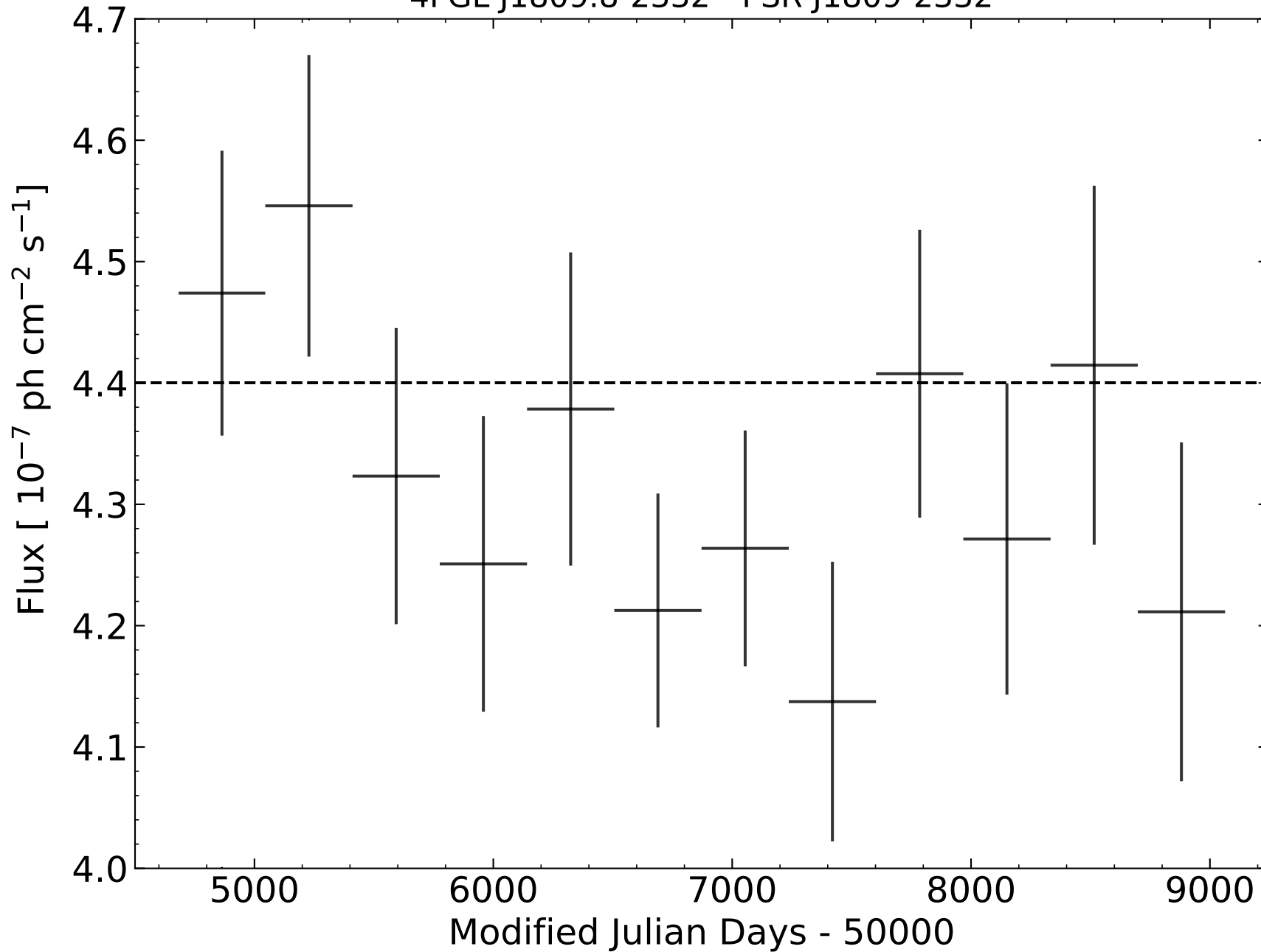
4FGL J1809.8-2332 - PSR J1809-2332
