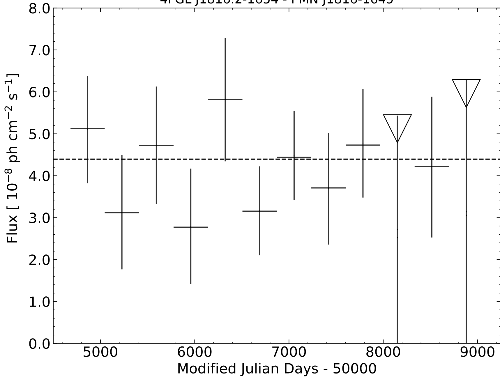
4FGL J1816.2-1654 - PMN J1816-1649
