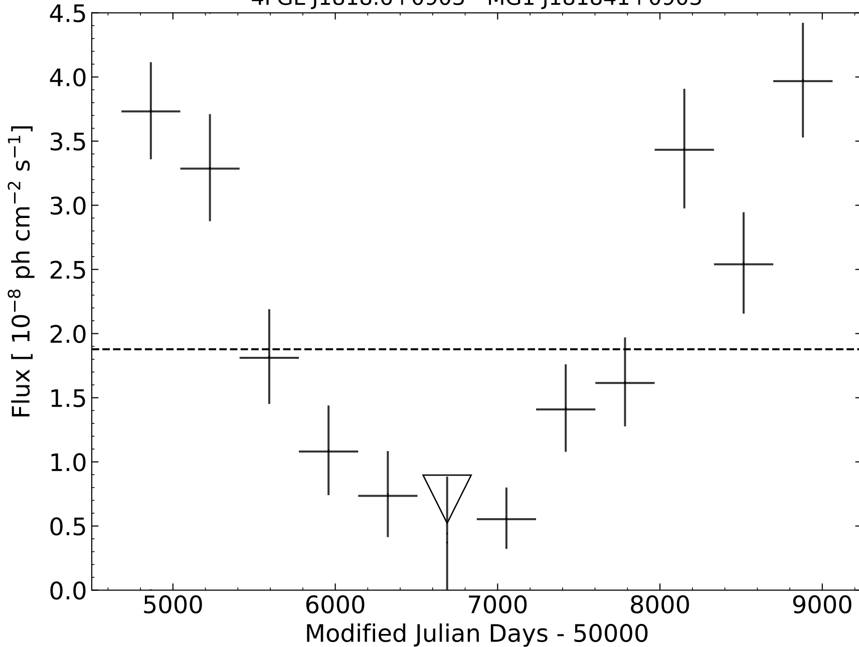
4FGL J1818.6+0903 - MG1 J181841+0903
