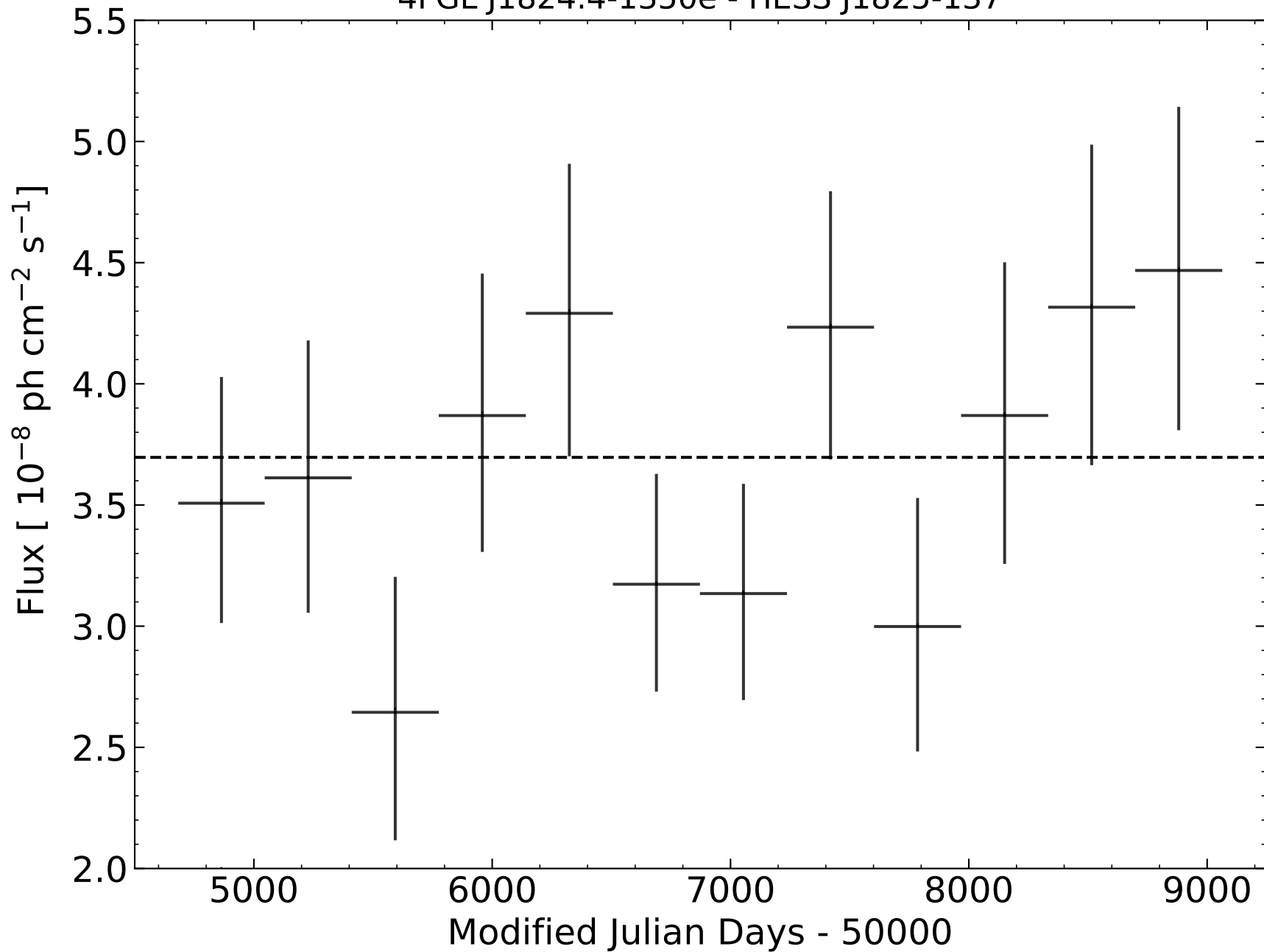
4FGL J1824.4-1350e - HESS J1825-137
