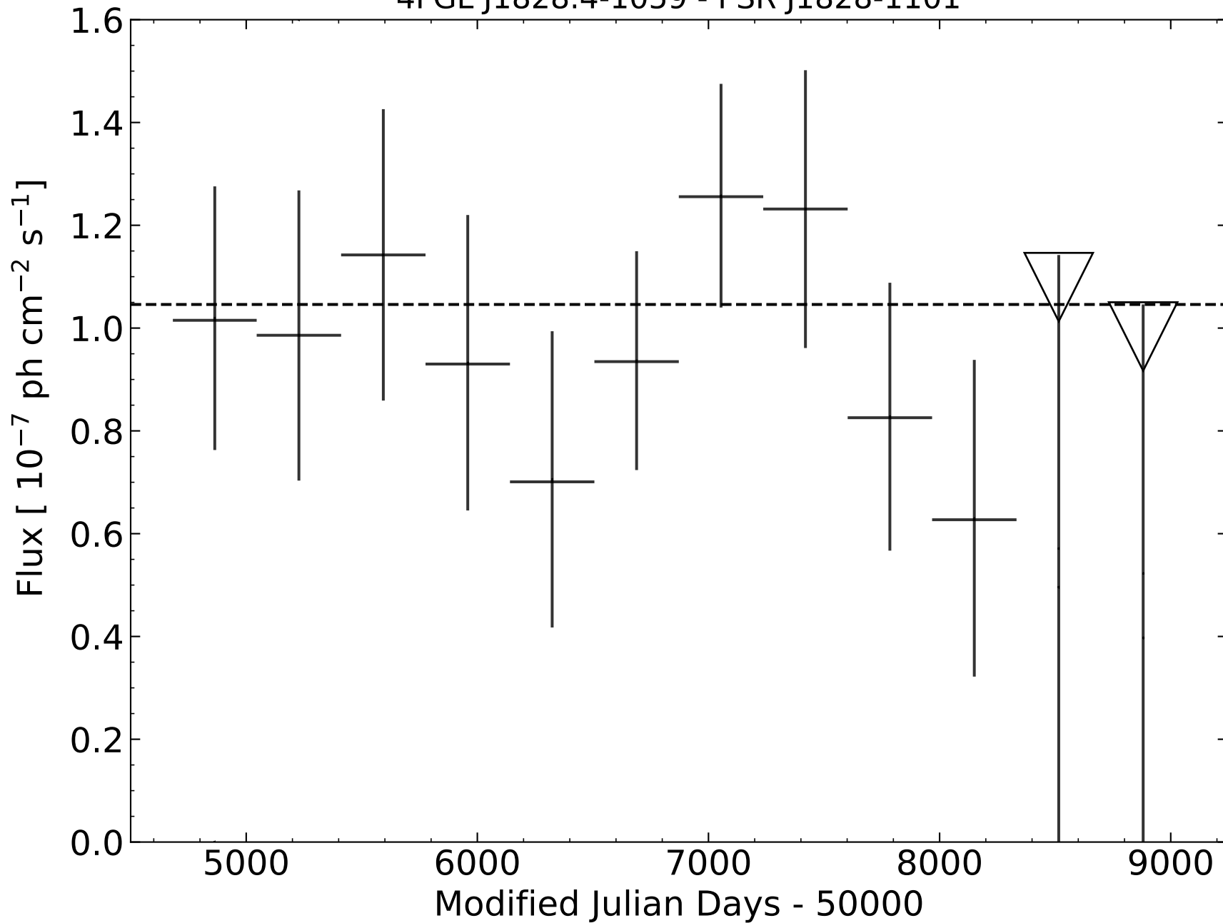
4FGL J1828.4-1059 - PSR J1828-1101
