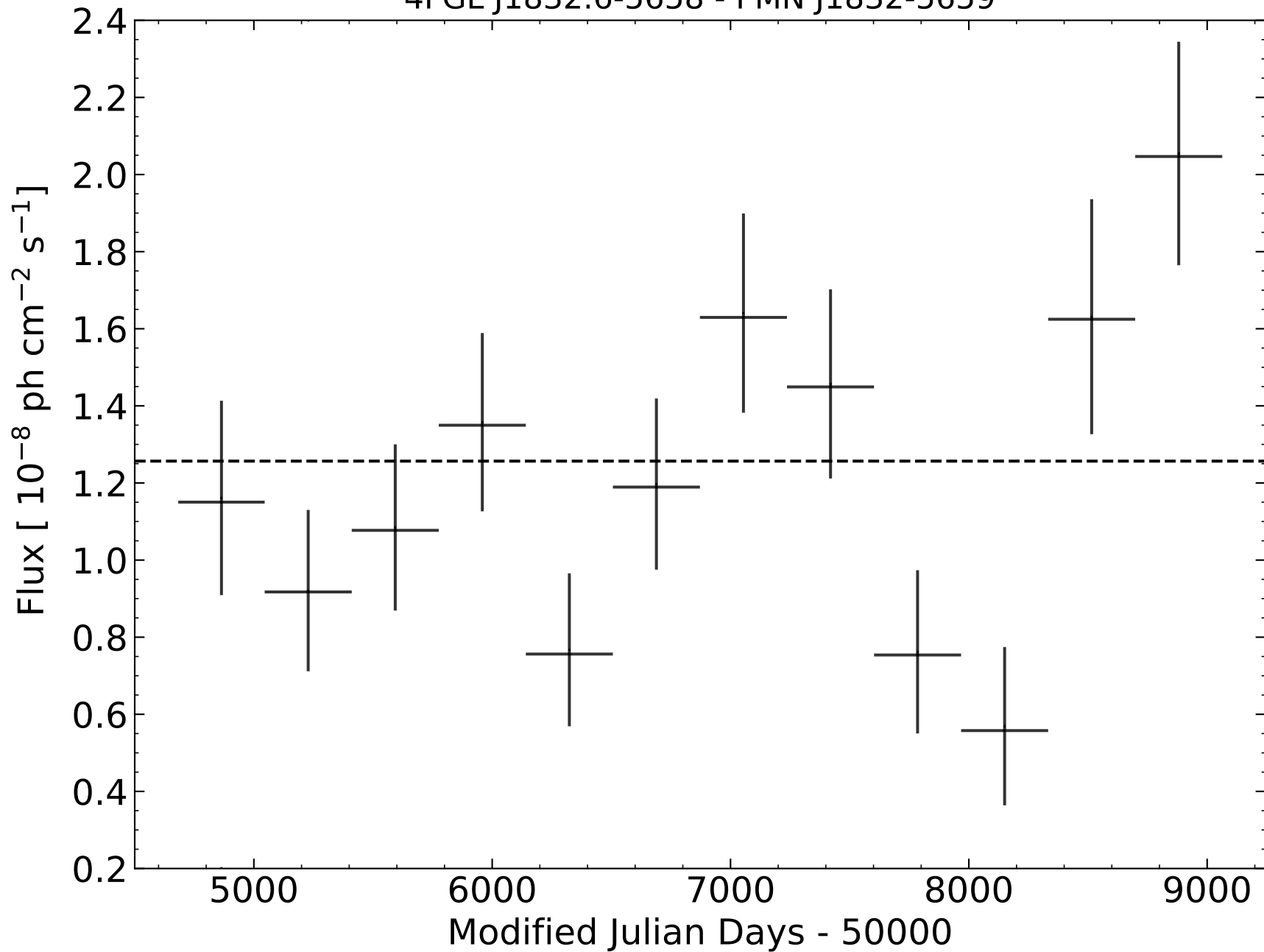
4FGL J1832.6-5658 - PMN J1832-5659
