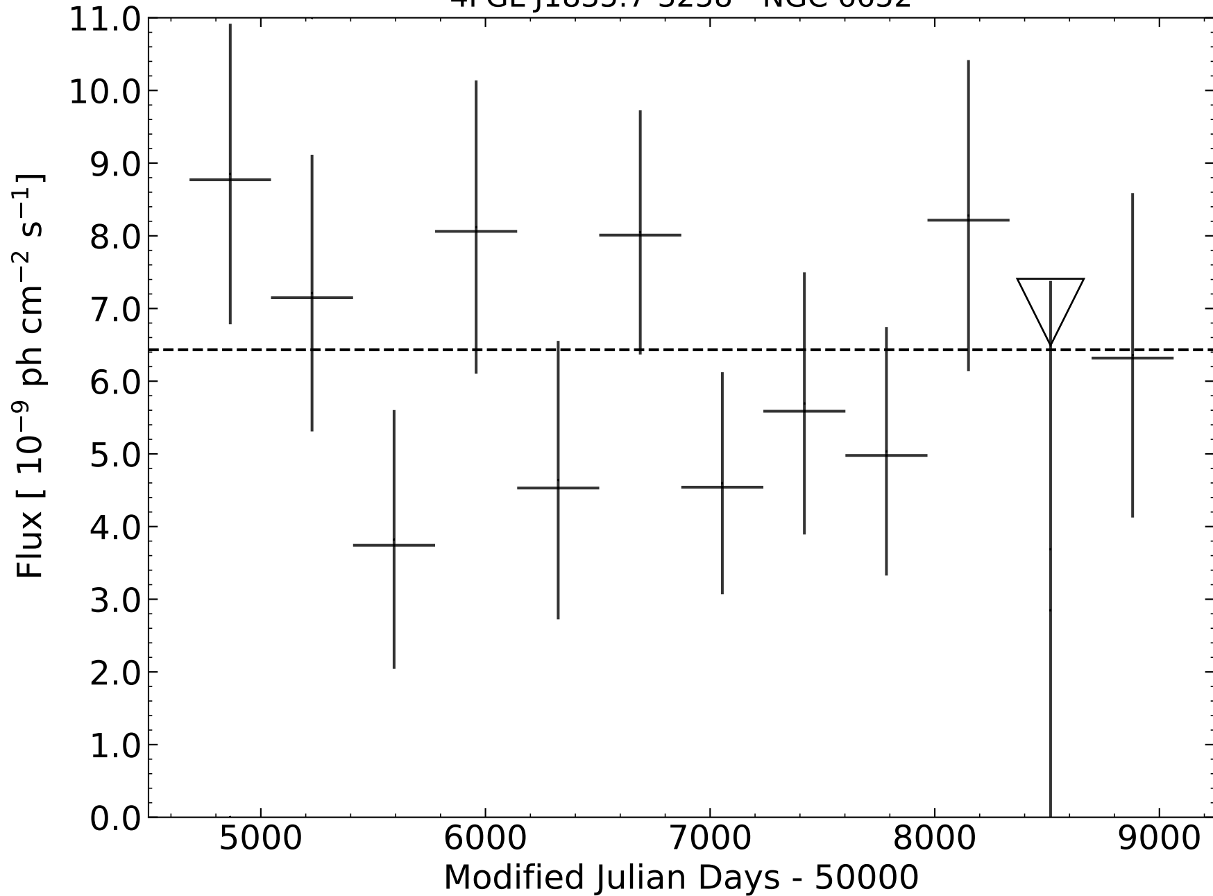
4FGL J1835.7-3258 - NGC 6652
