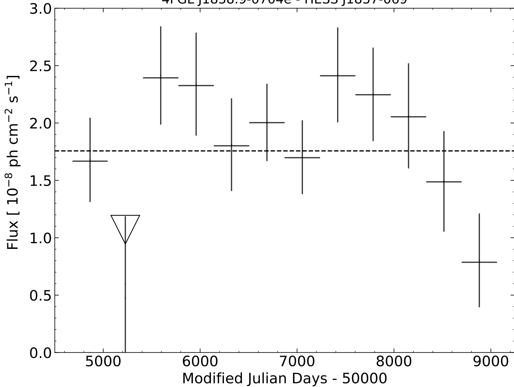
4FGL J1838.9-0704e - HESS J1837-069
