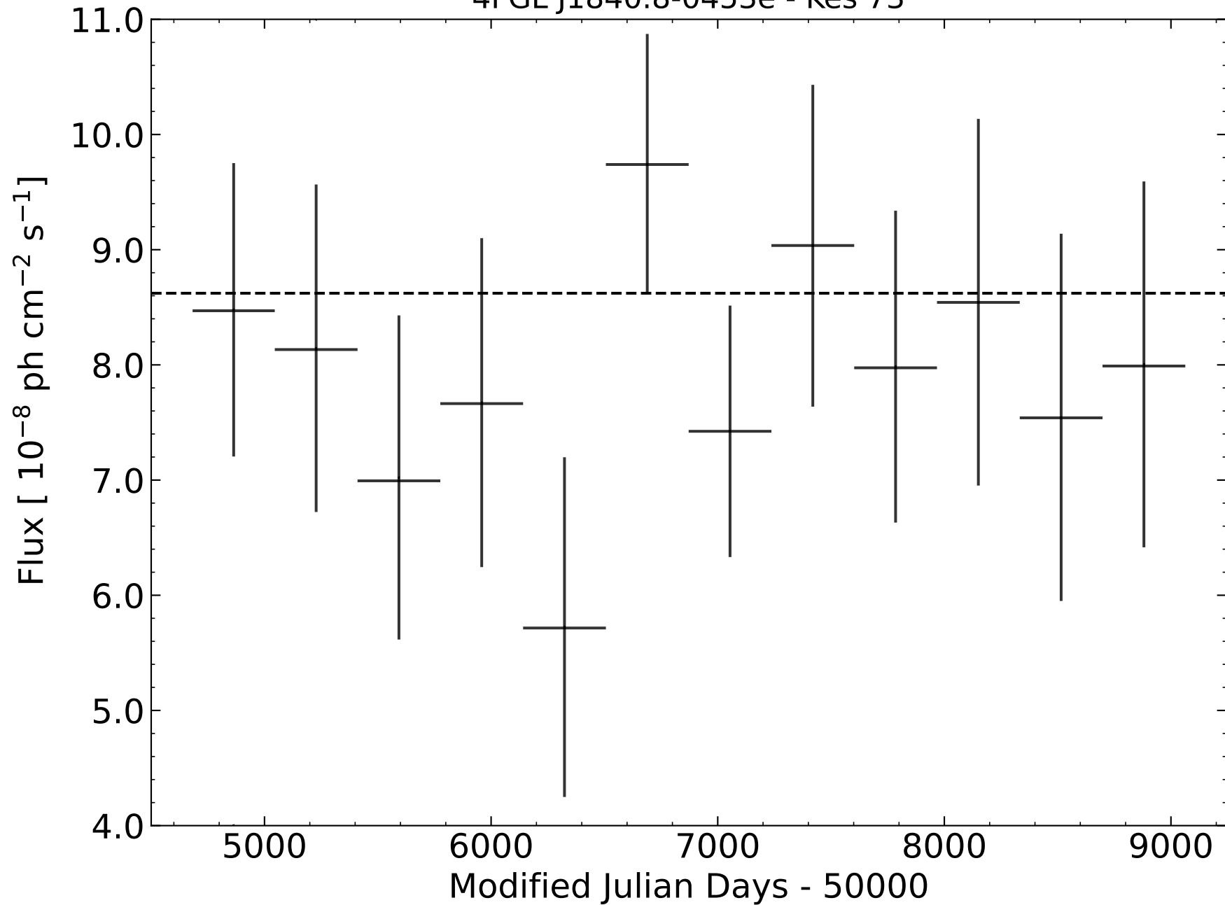
4FGL J1840.8-0453e - Kes 73
