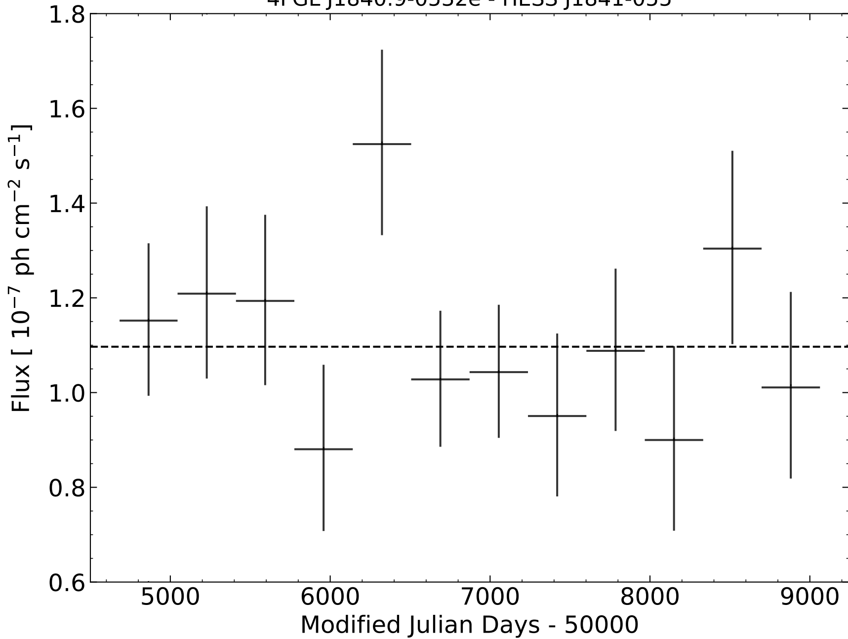
4FGL J1840.9-0532e - HESS J1841-055
