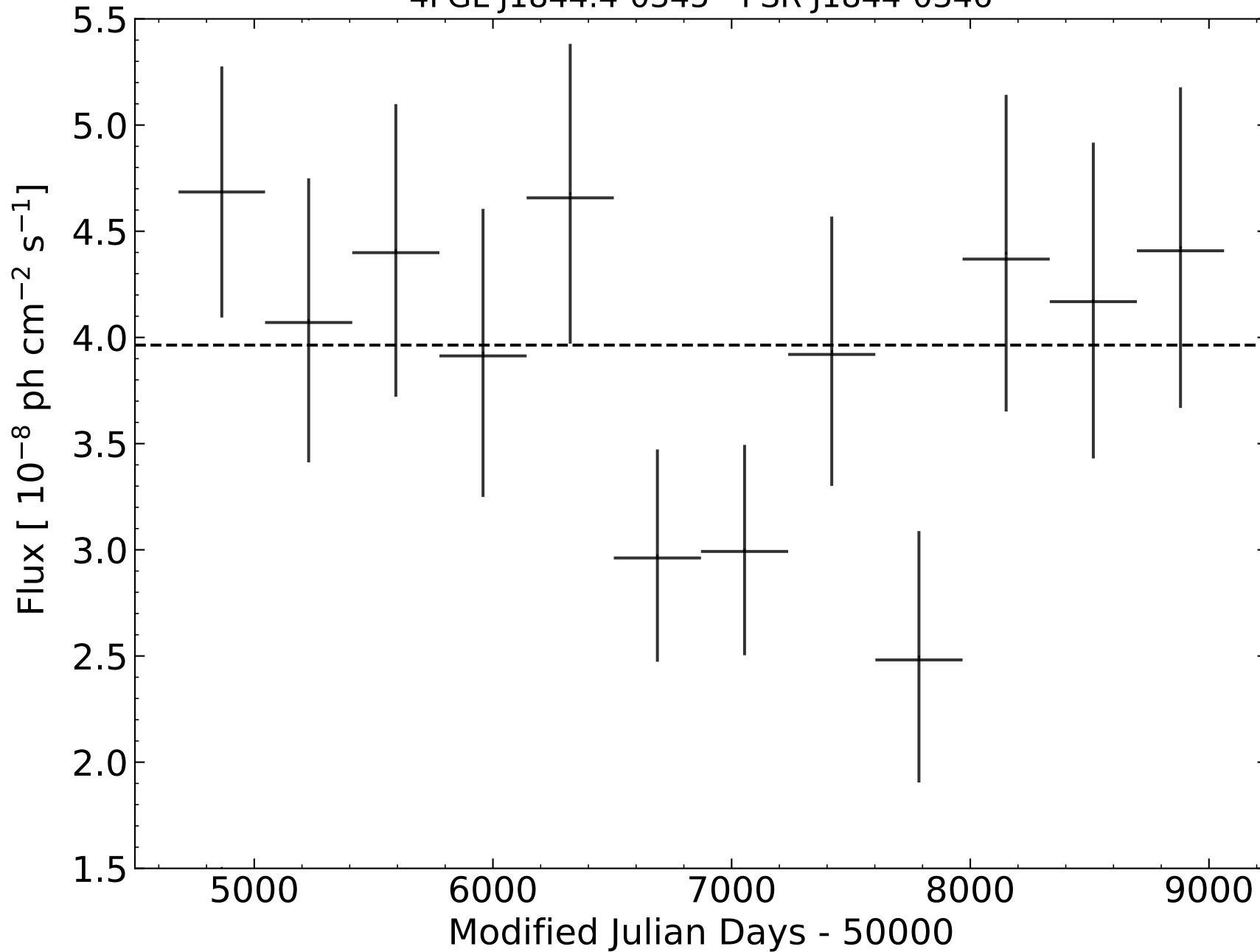
4FGL J1844.4-0345 - PSR J1844-0346
