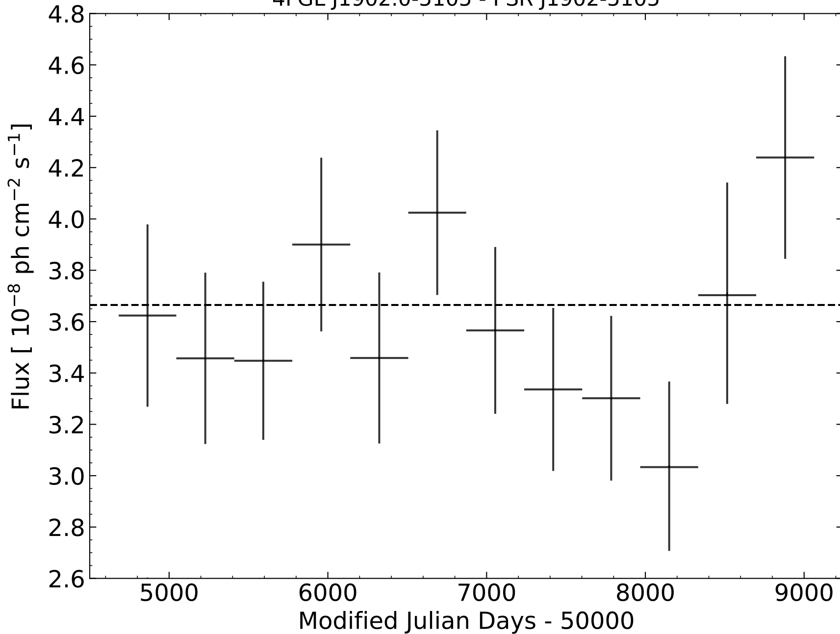
4FGL J1902.0-5105 - PSR J1902-5105
