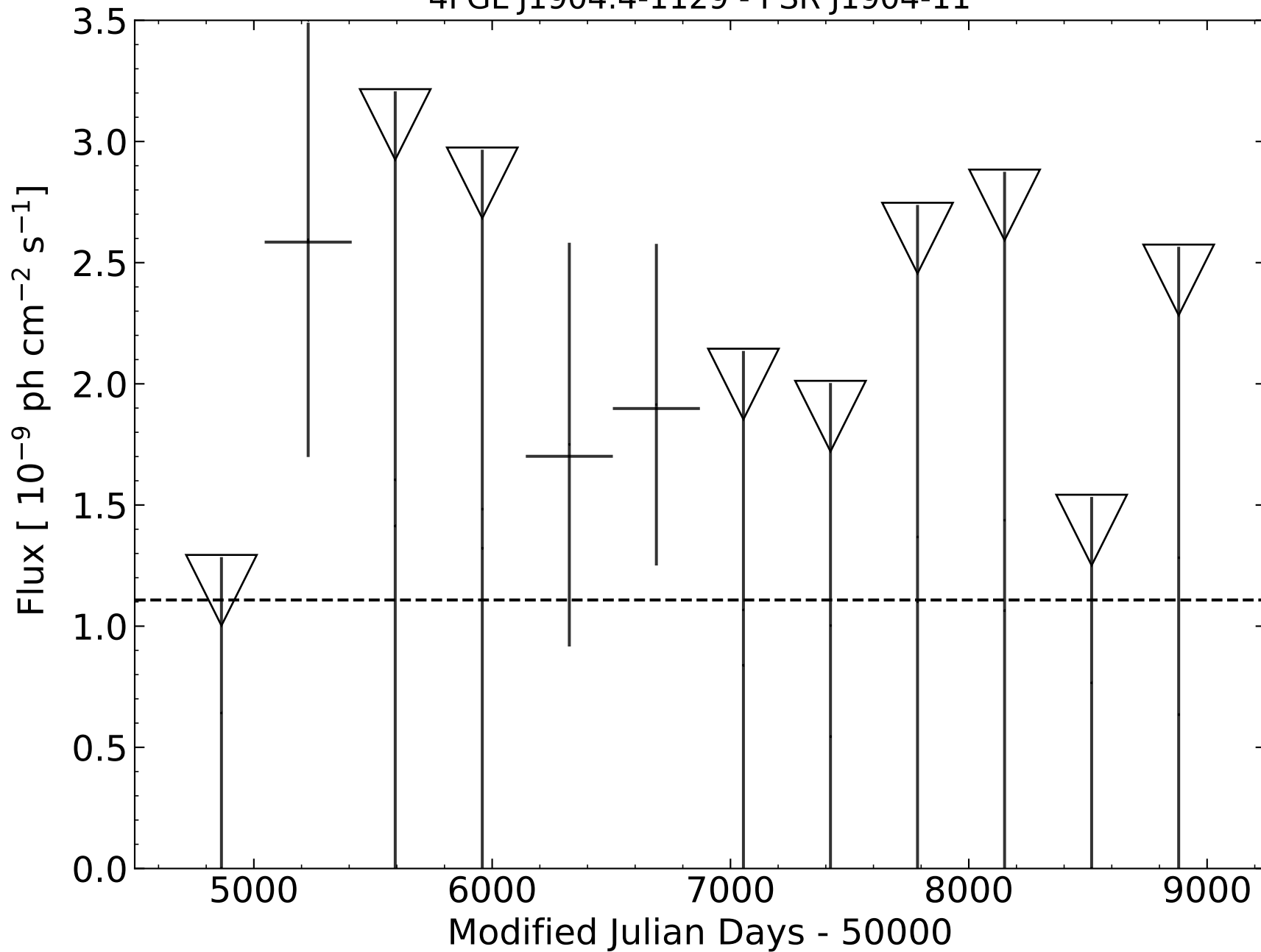
4FGL J1904.4-1129 - PSR J1904-11
